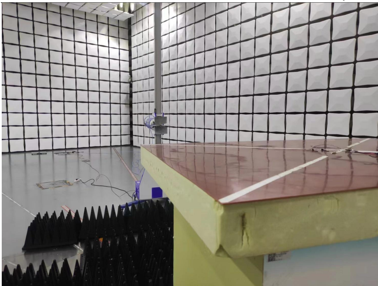
RE>1GHz
