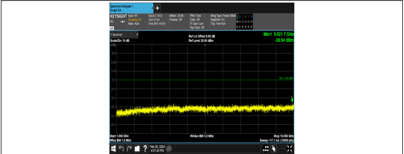
Band5-5MHz-16QAM-20525-1RB#0-Range2:1000~10000MHz
