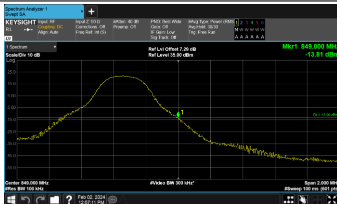
Band5-5MHz-QPSK-20625-25RB#0
