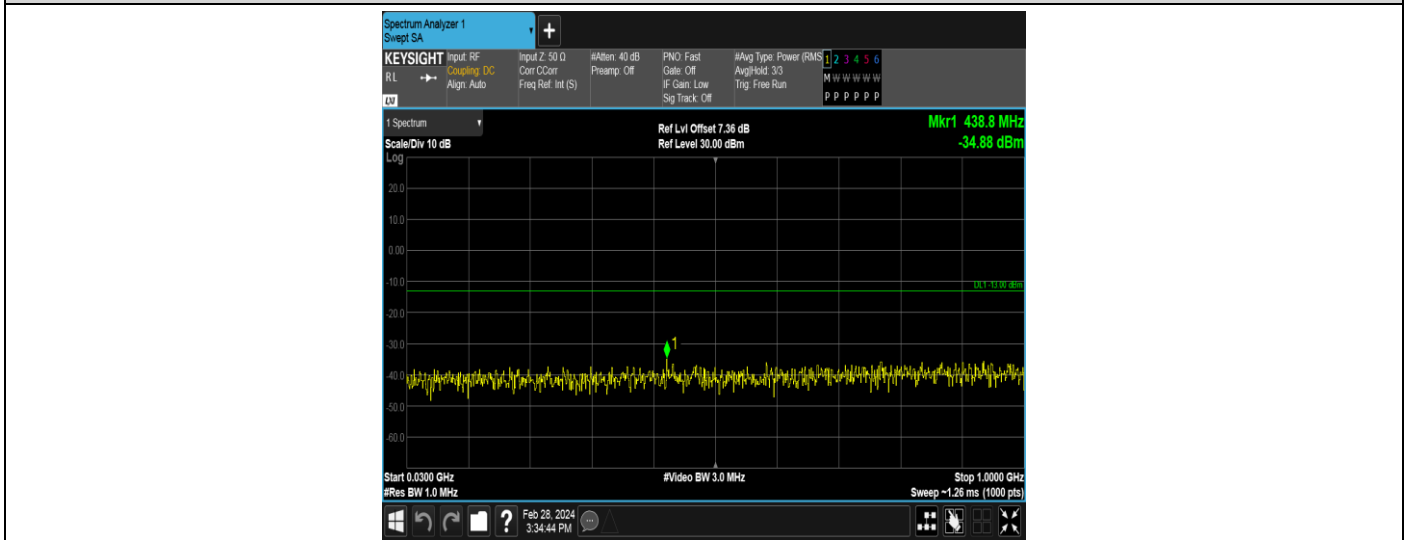
Band4-10MHz-16QAM-20175-1RB#0-Range1:30~1000MHz
