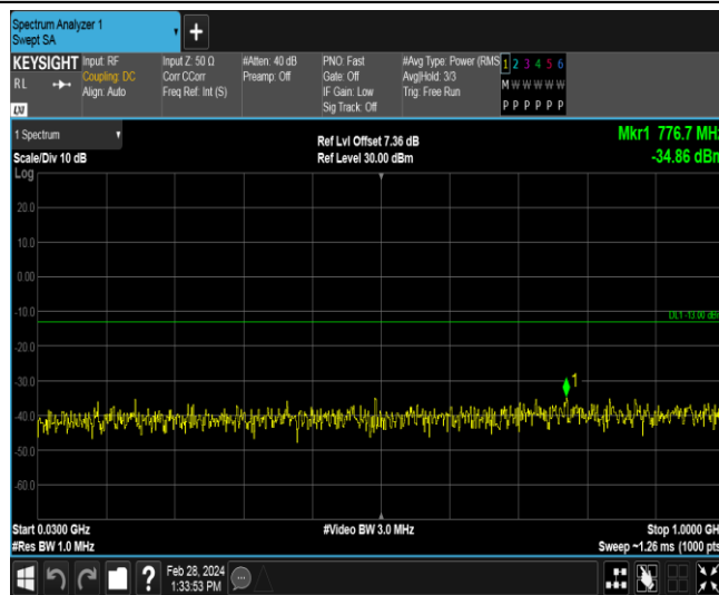
Band2-3MHz-QPSK-18615-1RB#0-Range1:30~1000MHz
