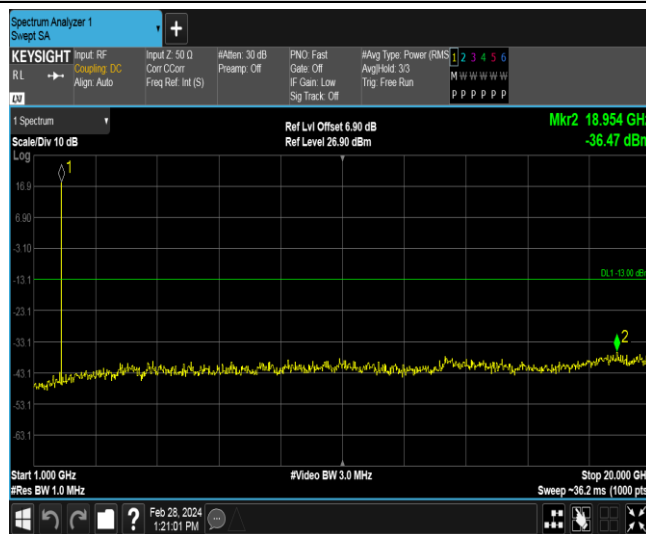
Band2-1.4MHz-16QAM-18607-1RB#0-Range2:1000~20000MHz
