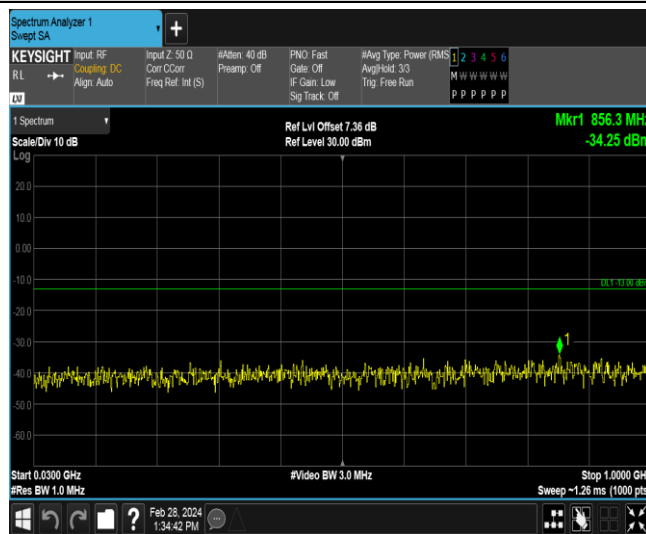
Band2-3MHz-16QAM-19185-1RB#0-Range1:30~1000MHz
