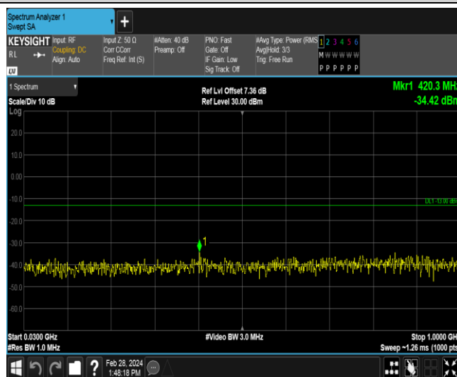
Band2-5MHz-16QAM-18900-1RB#0-Range1:30~1000MHz
