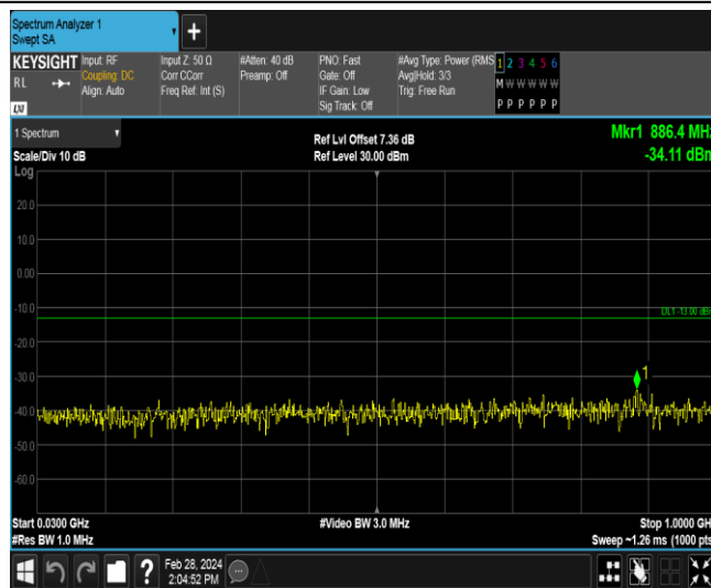
Band2-10MHz-16QAM-18650-1RB#0-Range1:30~1000MHz
