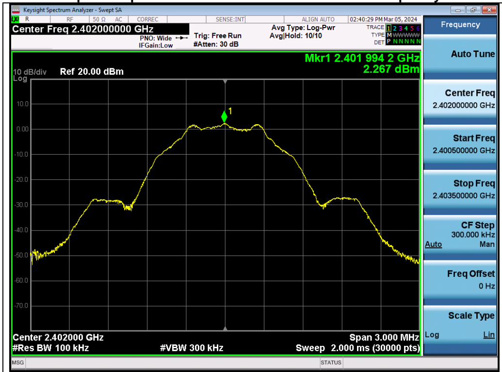
Test_Graph_LE1M_ANT1_2402_1Mbps_Reference Level
