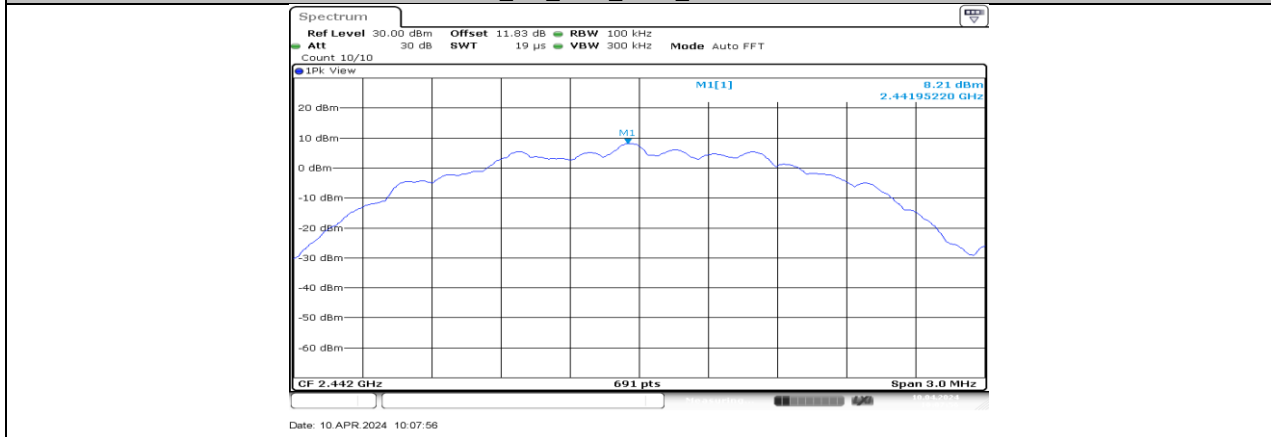
BLE_2M_Ant1_2442_0~Reference
