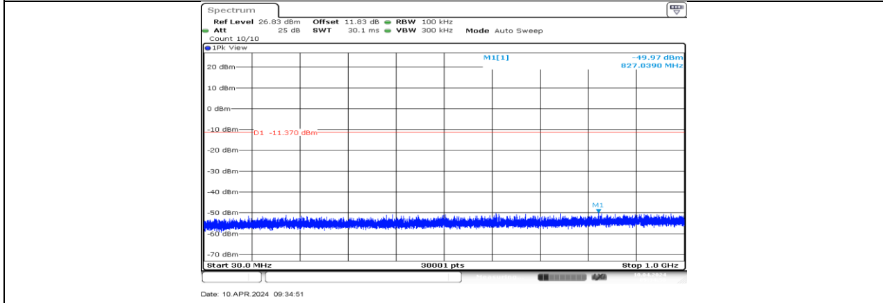
BLE_1M_Ant1_2442_30~1000
