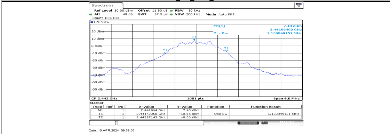
BLE_1M_Ant1_2442
