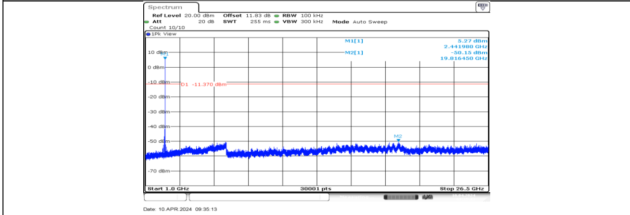
BLE_1M_Ant1_2442_1000~26500
