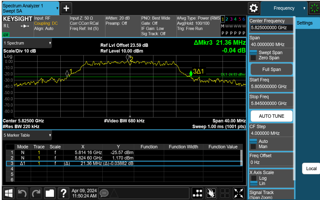
11AC20SISO-Ant1-5825
