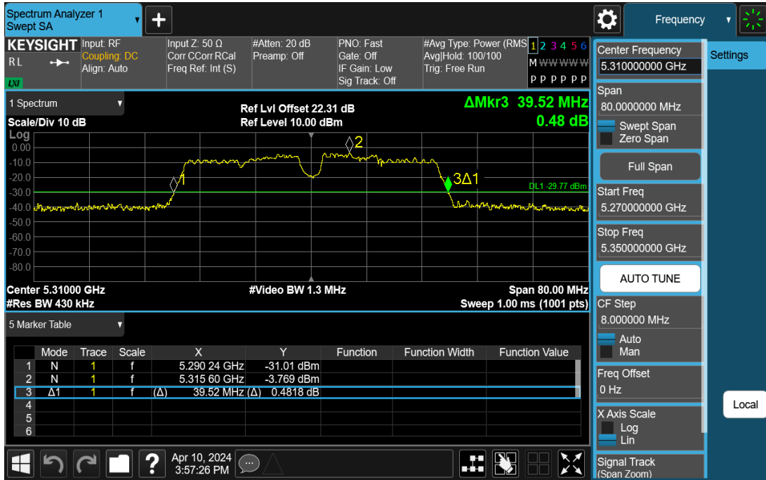
11AC40SISO-Ant1-5310
