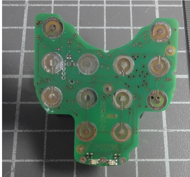
PCB, bottom view*
