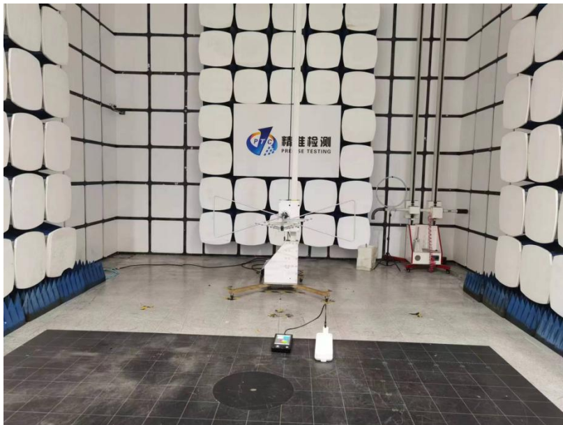
Radiated Emissions Test Frequency From 30MHz-1GHz
