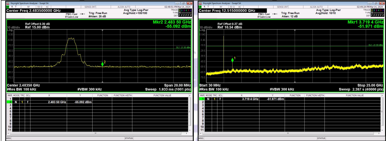
Out Of Band Emission LE_Channel 39
