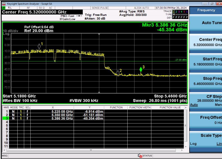
11AX160SISO-Ant3-5250-PASS
