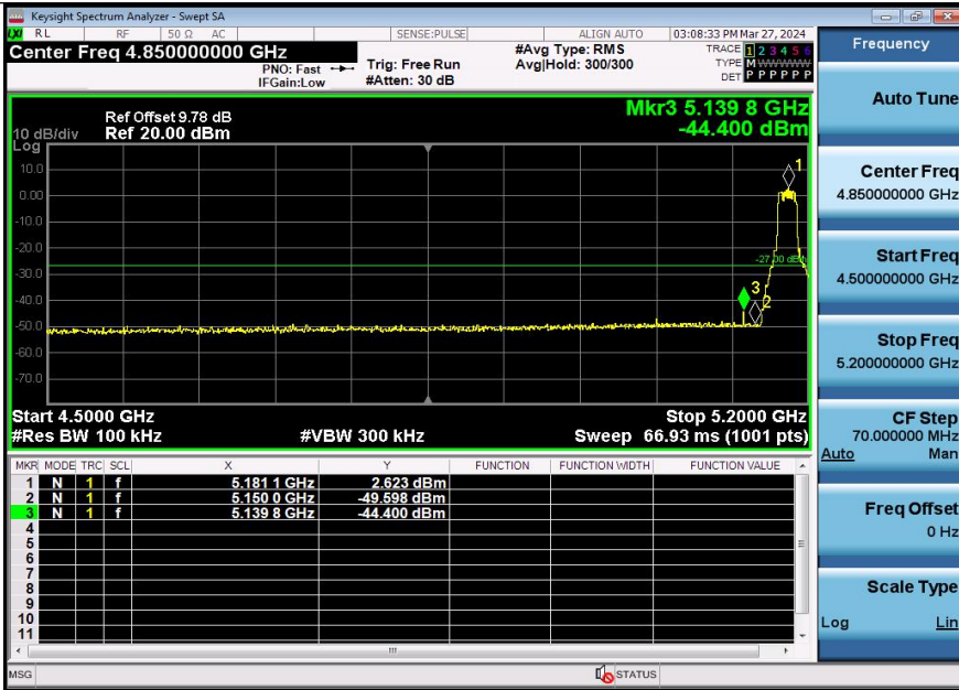
11AX20SISO-Ant3-5180-PASS
