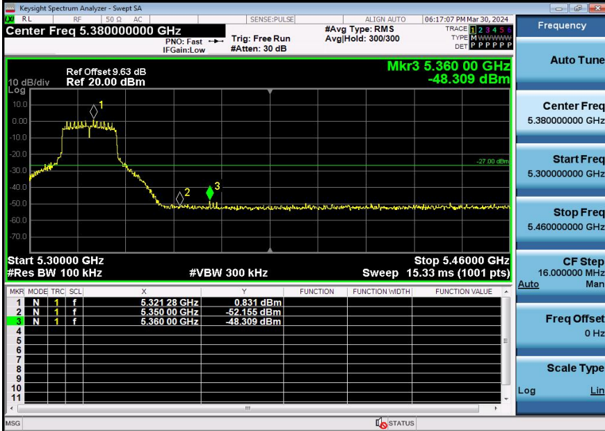
11AX20SISO-Ant3-5320-PASS
