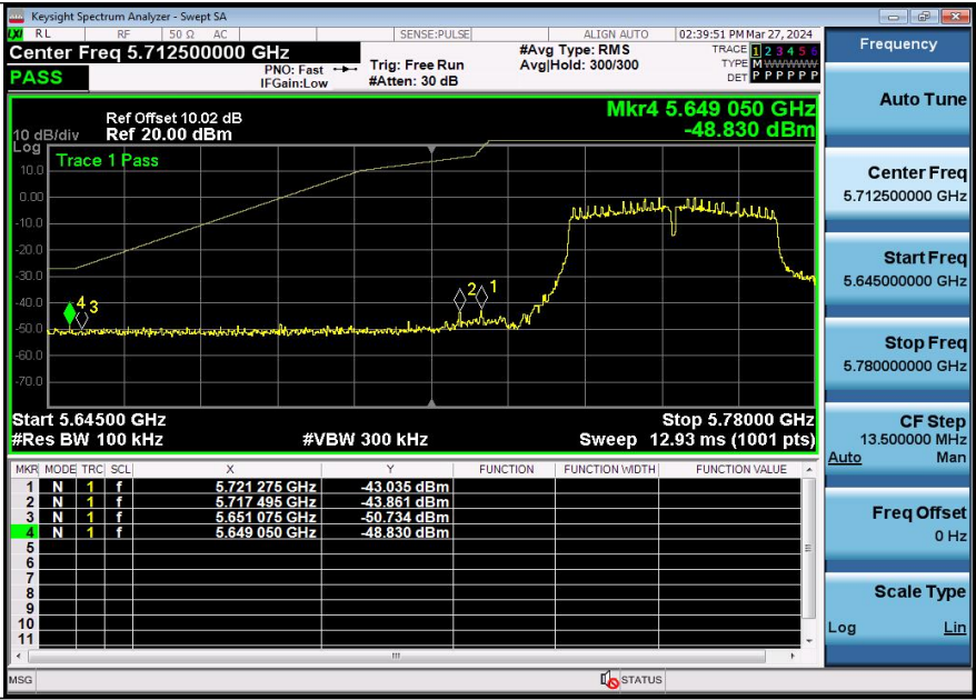
11AC40SISO-Ant3-5755-PASS
