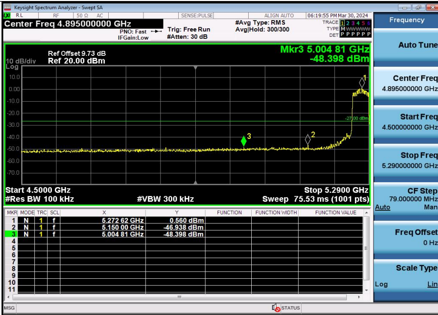
11AX40SISO-Ant3-5270-PASS
