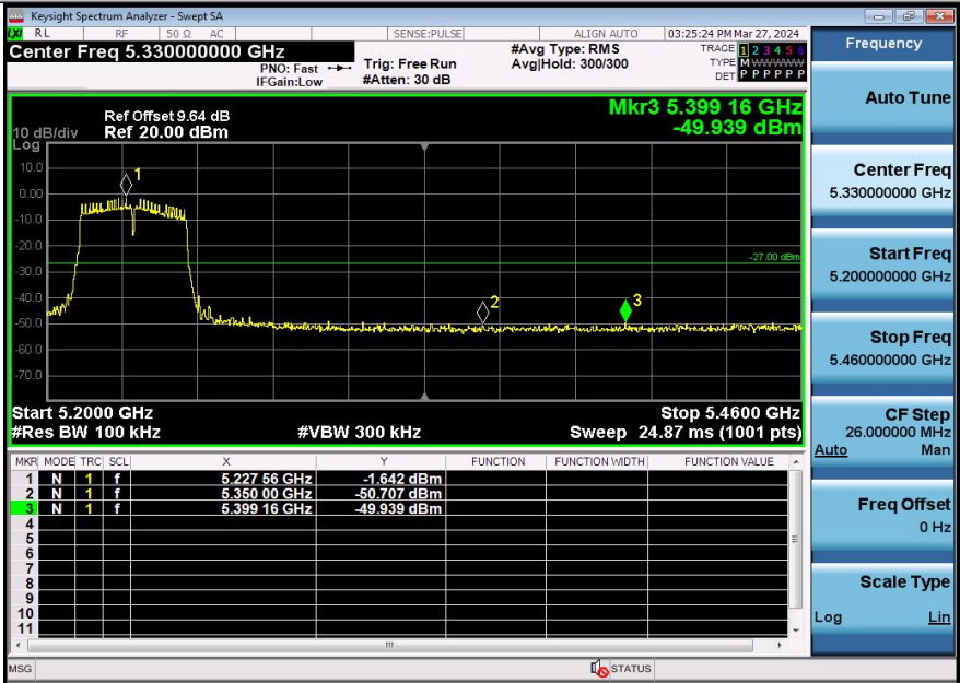
11AX40SISO-Ant3-5230-PASS
