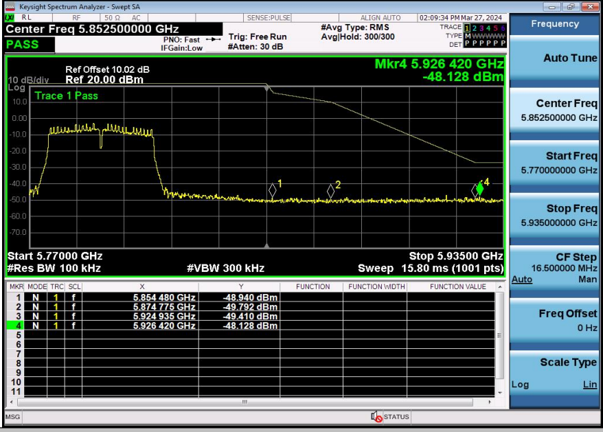
11N40ISO-Ant3-5795-PASS
