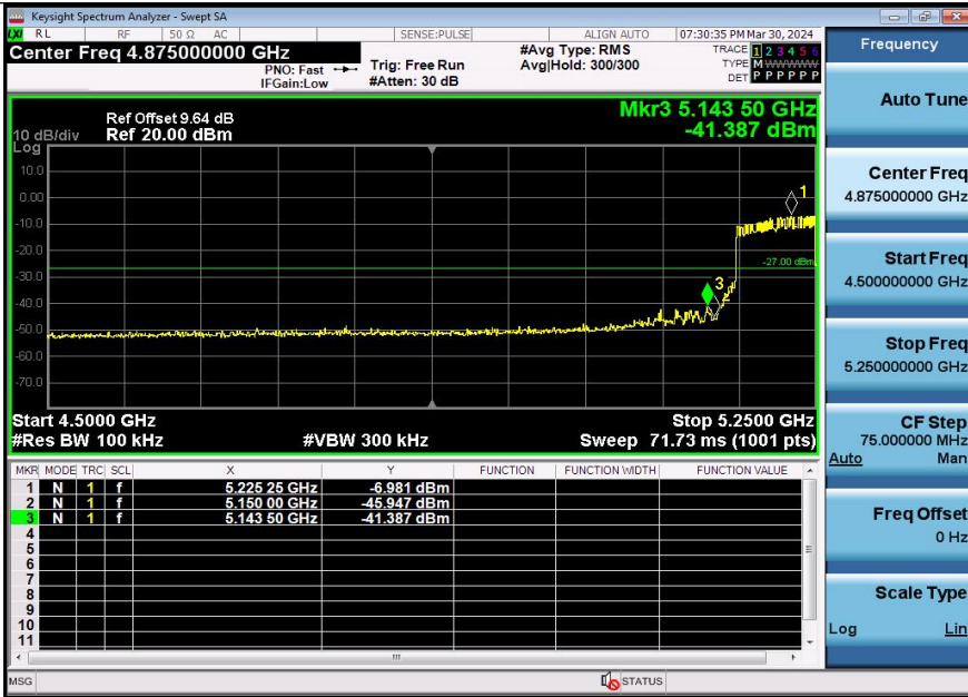
11AX160SISO-Ant3-5250-PASS
