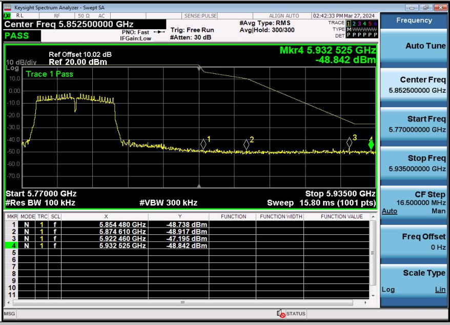
11AC40SISO-Ant3-5795-PASS
