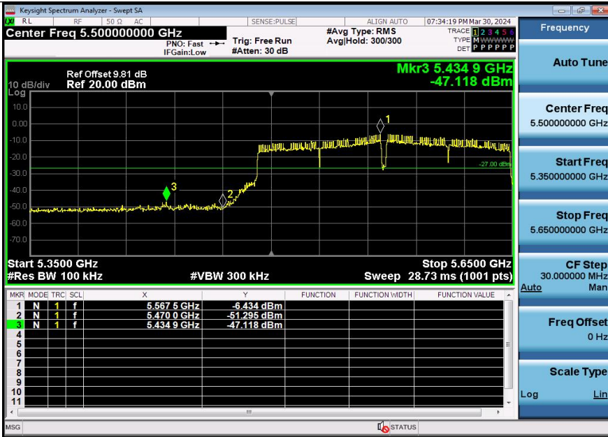
11AX160SISO-Ant3-5570-PASS
