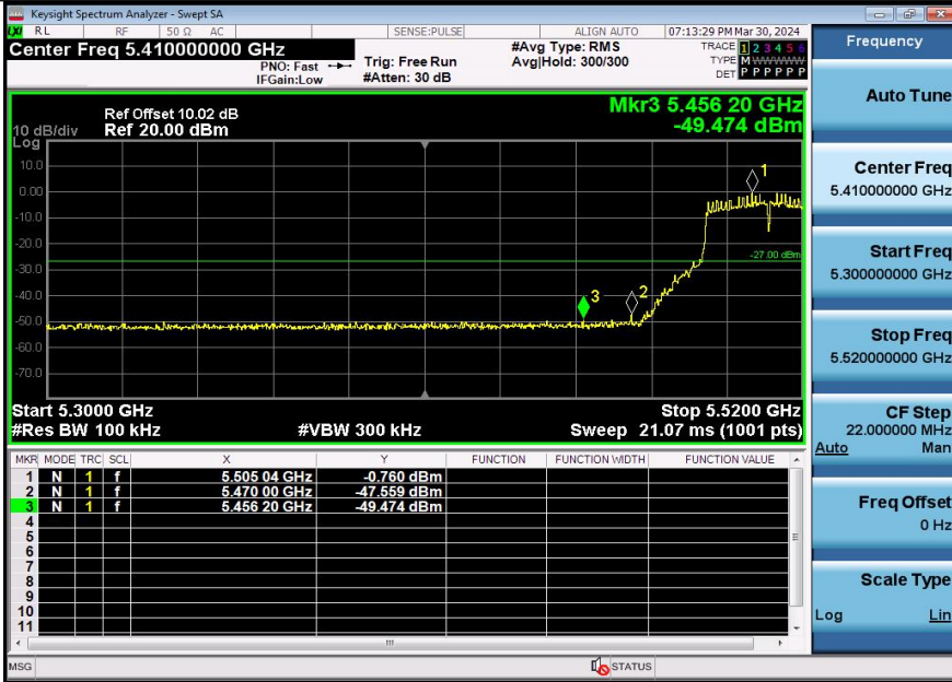
11AX40SISO-Ant3-5510-PASS
