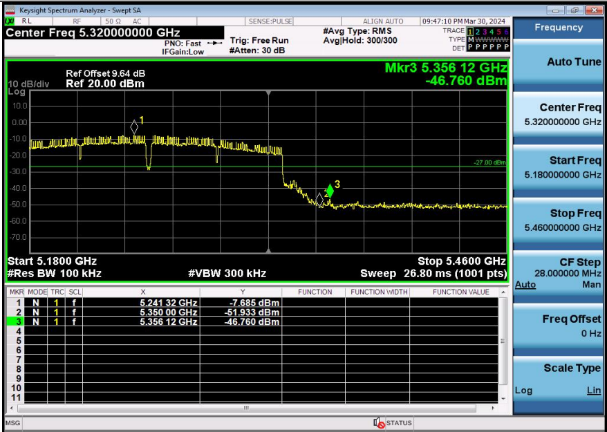
11AX160SISO-Ant1-5250-PASS
