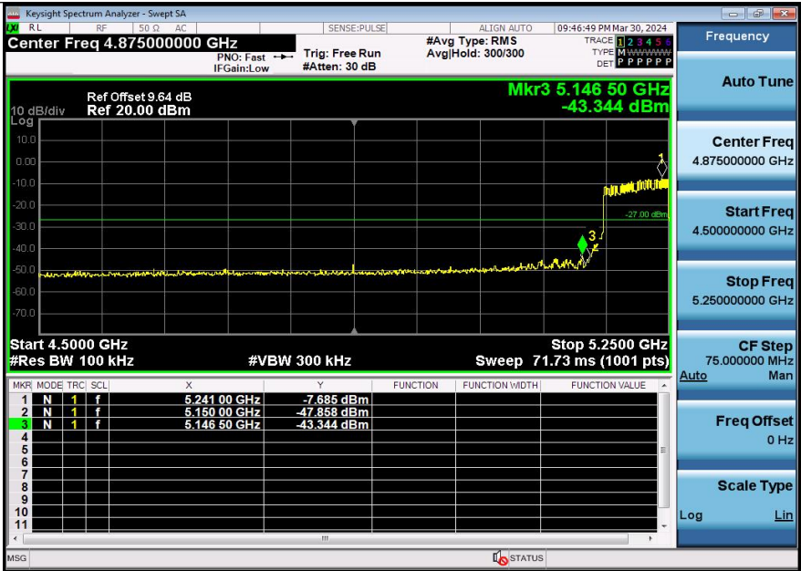
11AX160SISO-Ant1-5250-PASS
