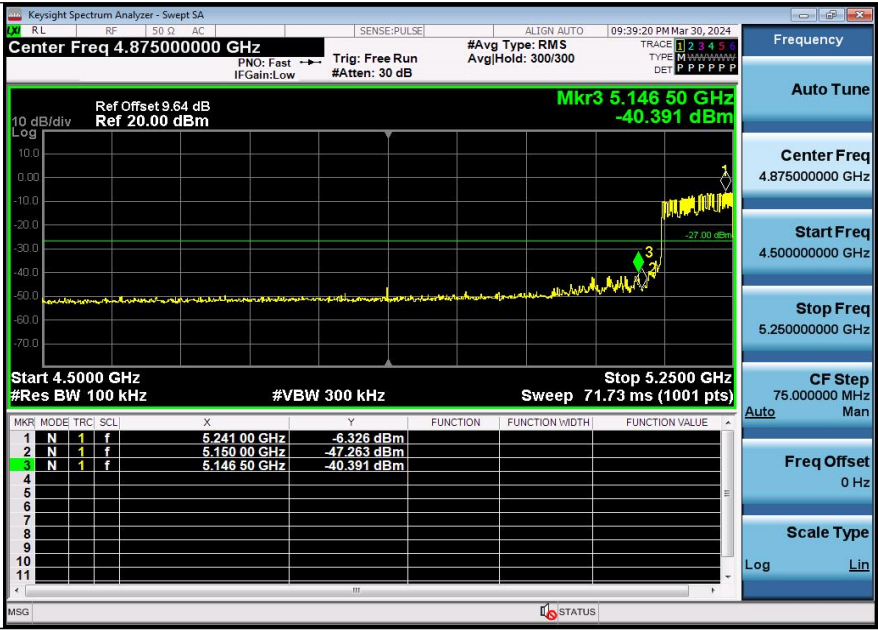
11AC160SISO-Ant1-5250-PASS
