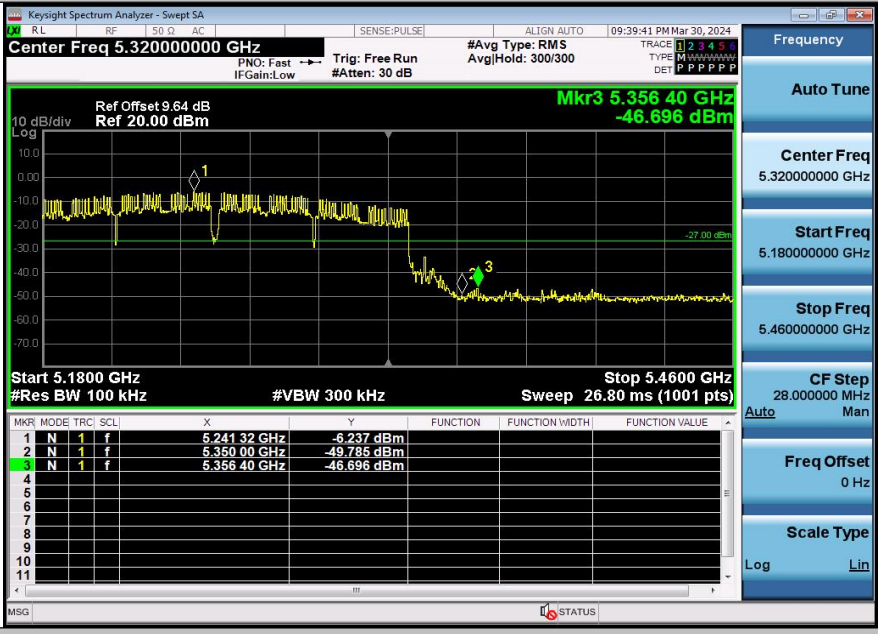
11AC160SISO-Ant1-5250-PASS
