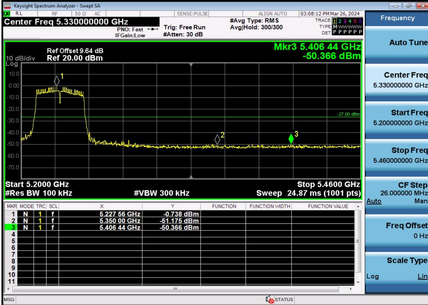
11AX40SISO-Ant1-5230-PASS
