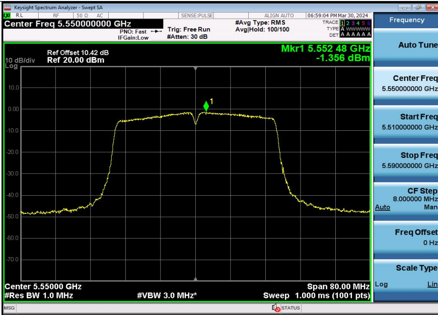
11AC40SISO-Ant3-5550-PASS
