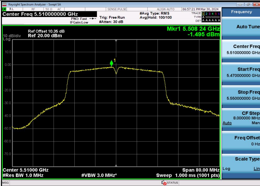
11AC40SISO-Ant3-5510-PASS
