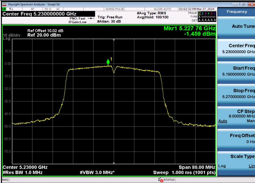
11N40SISO-Ant3-5230-PASS
