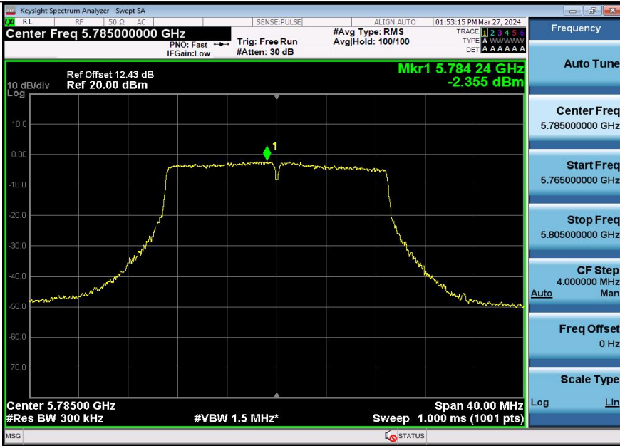
11N20SISO-Ant3-5785-PASS
