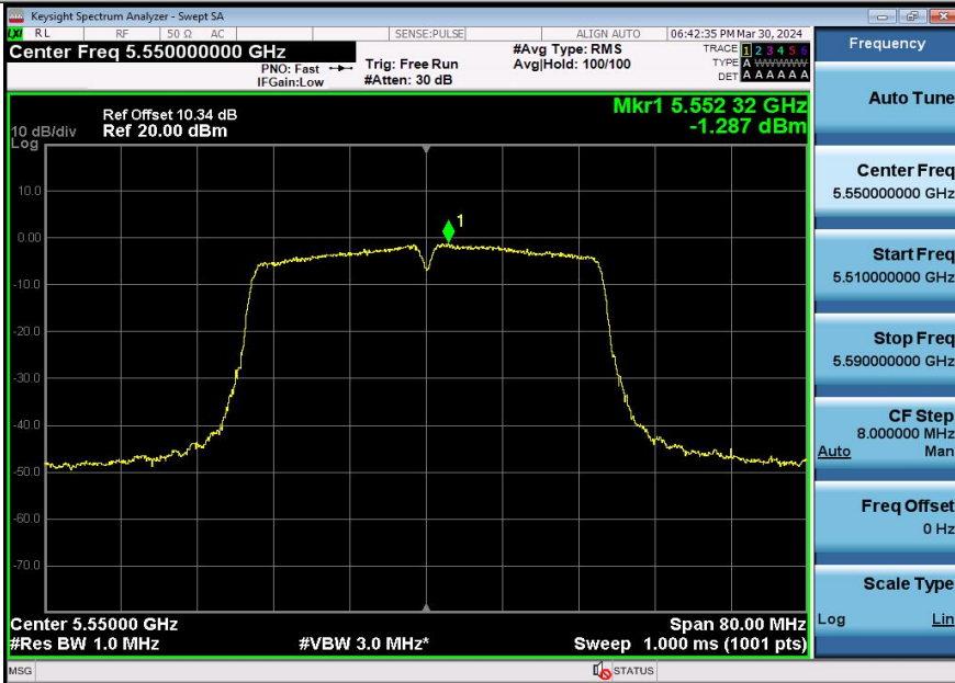
11N40SISO-Ant3-5550-PASS
