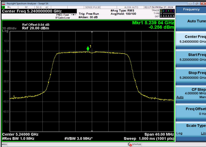
11AC20SISO-Ant3-5240-PASS
