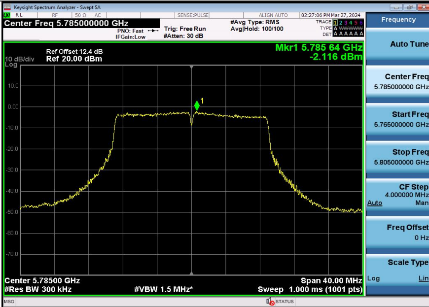
11AC20SISO-Ant3-5785-PASS
