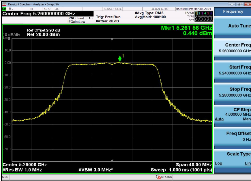
11AC20SISO-Ant3-5260-PASS
