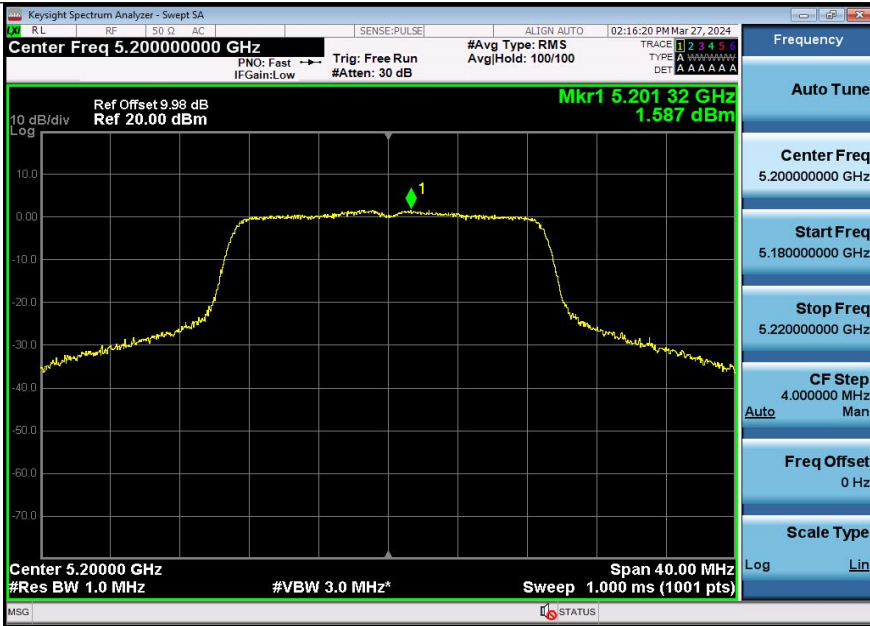
11AC20SISO-Ant3-5200-PASS
