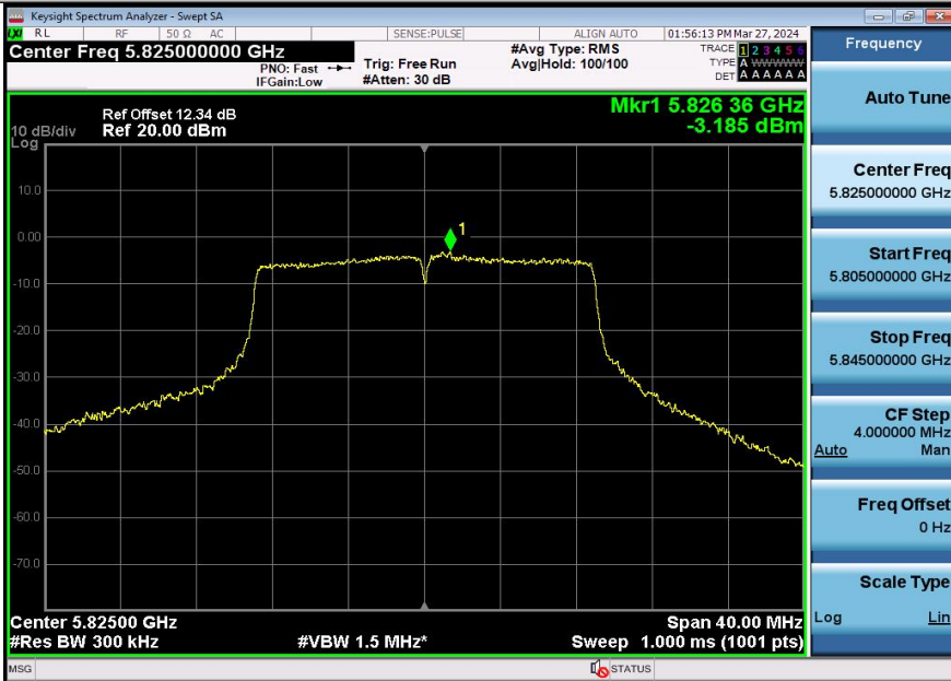
11N20SISO-Ant3-5825-PASS
