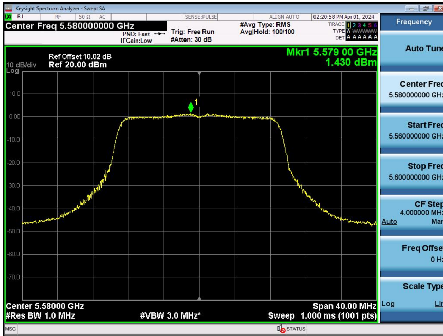
11AC20SISO-Ant3-5580-PASS
