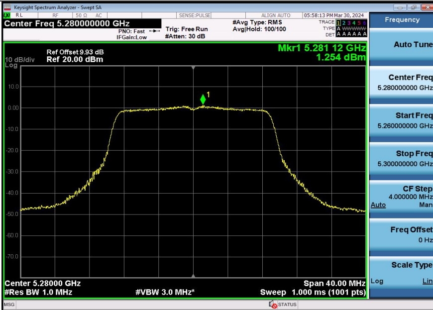
11AC20SISO-Ant3-5280-PASS
