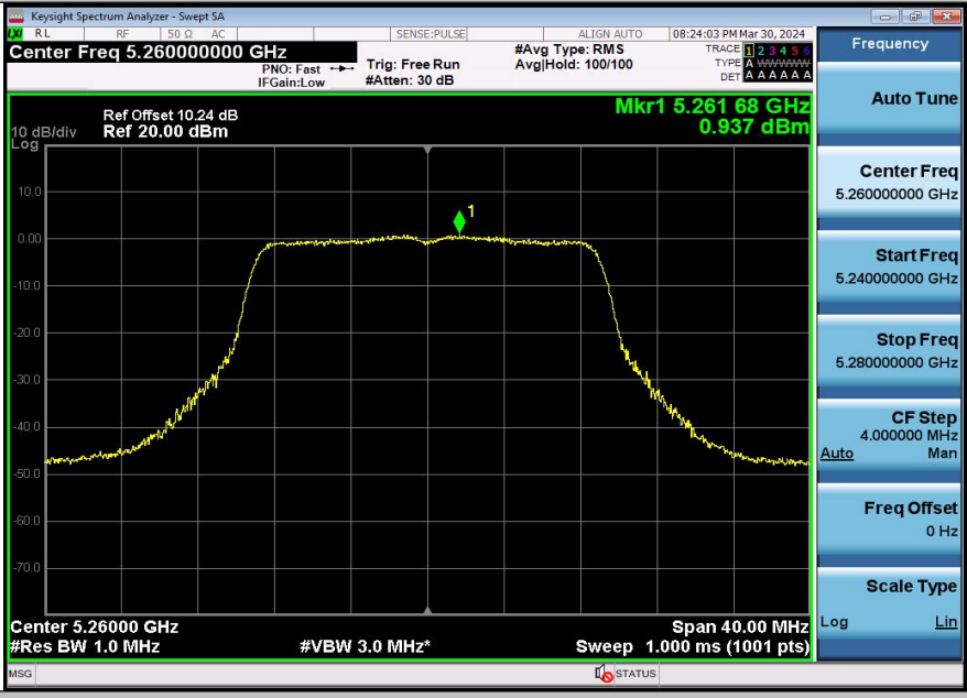
11AX20SISO-Ant1-5260-PASS
