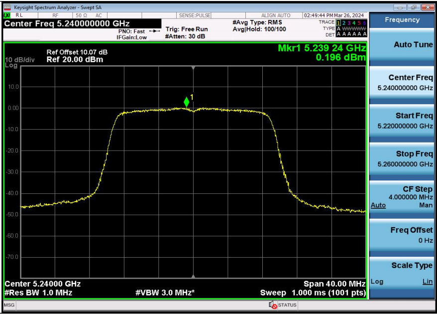
11AX20SISO-Ant1-5240-PASS
