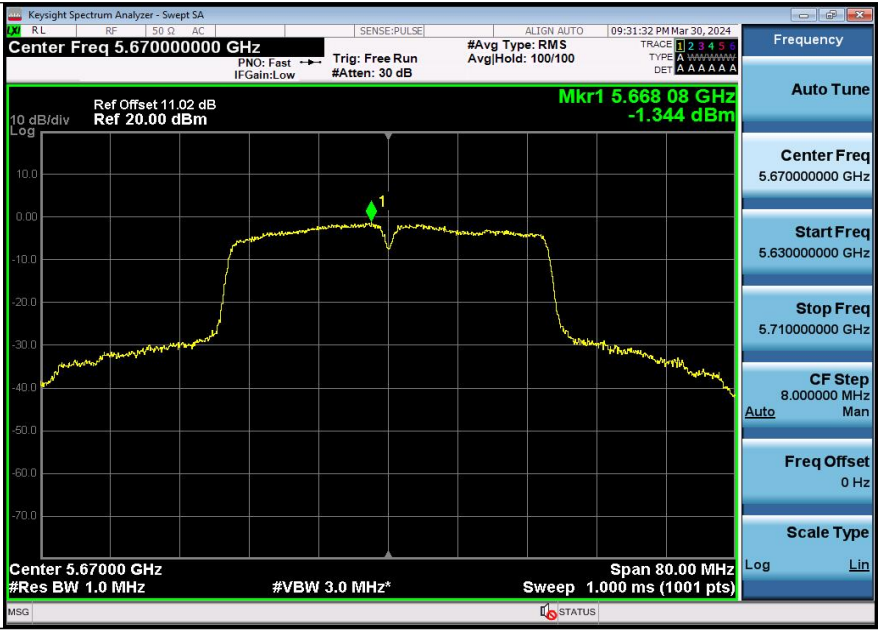
11AX40SISO-Ant1-5670-PASS
