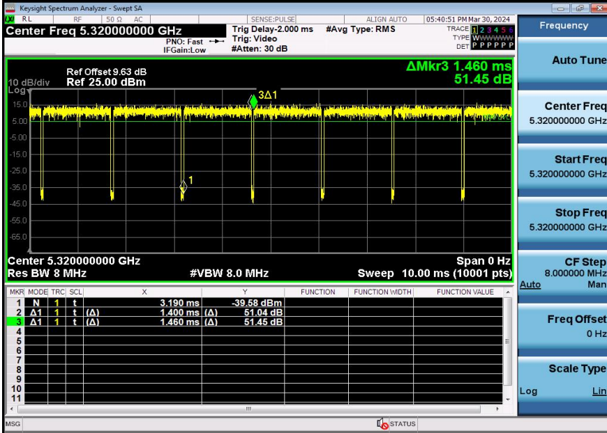
NTNV-11A-Ant3-5320
