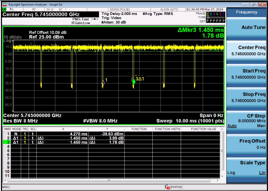
NTNV-11A-Ant3-5745
