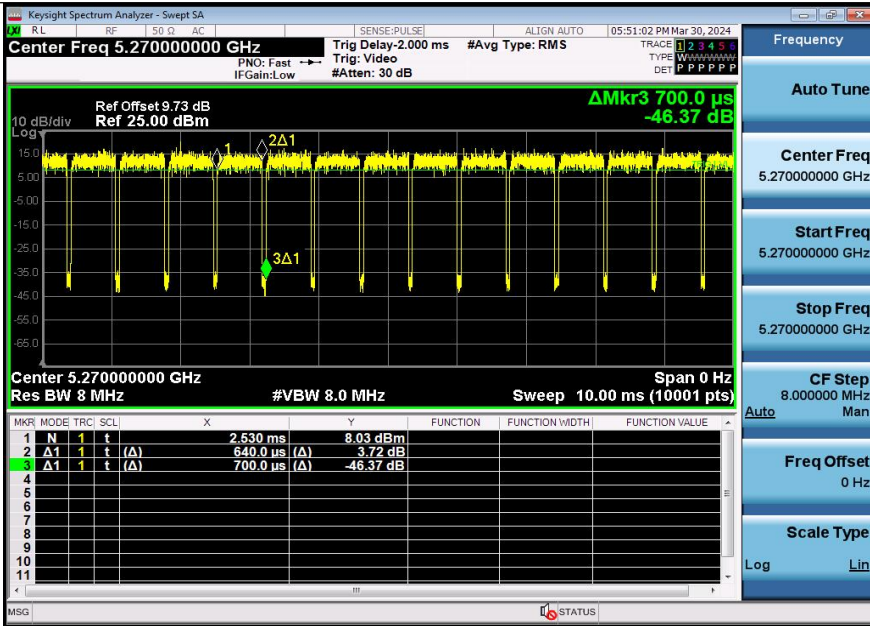
NTNV-11N40SISO-Ant3-5270
