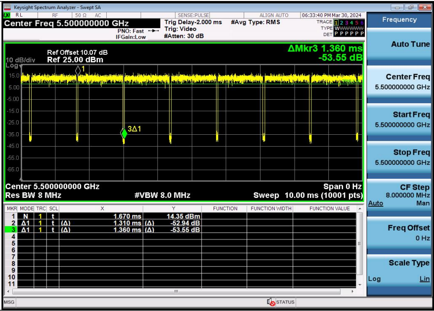
NTNV-11N20SISO-Ant3-5500
