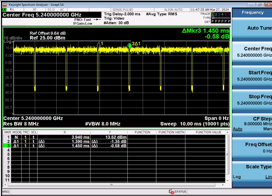
NTNV-11A-Ant3-5240
