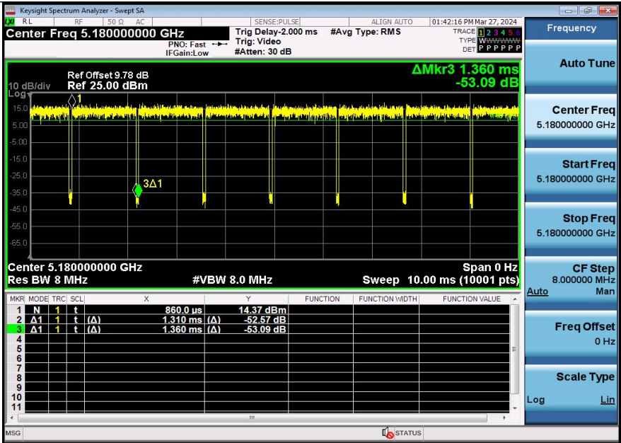
NTNV-11N20SISO-Ant3-5180
