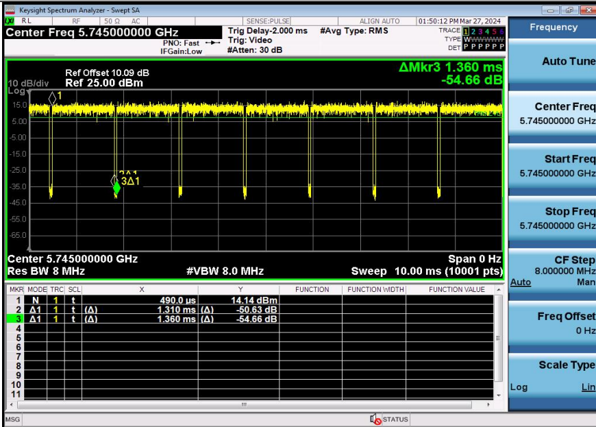
NTNV-11N20SISO-Ant3-5745
