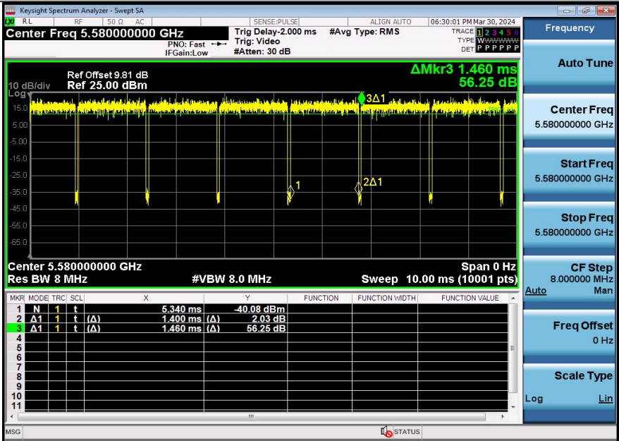
NTNV-11A-Ant3-5580
