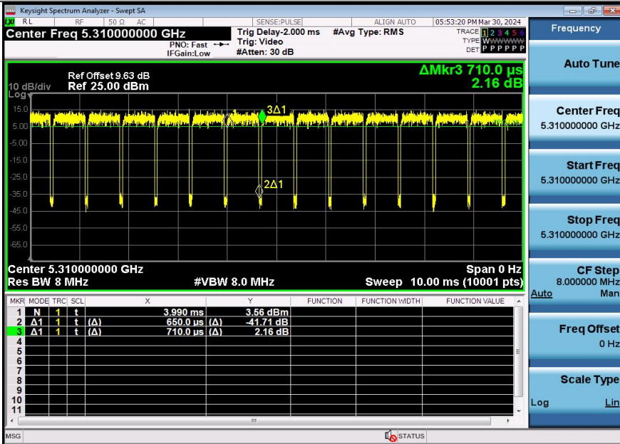
NTNV-11N40SISO-Ant3-5310
