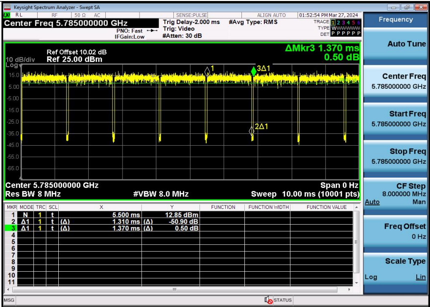
NTNV-11N20SISO-Ant3-5785
