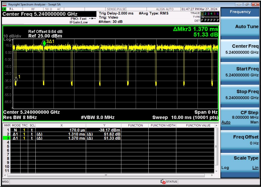
NTNV-11N20SISO-Ant3-5240
