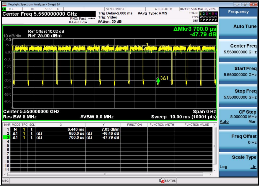
NTNV-11N40SISO-Ant3-5550
