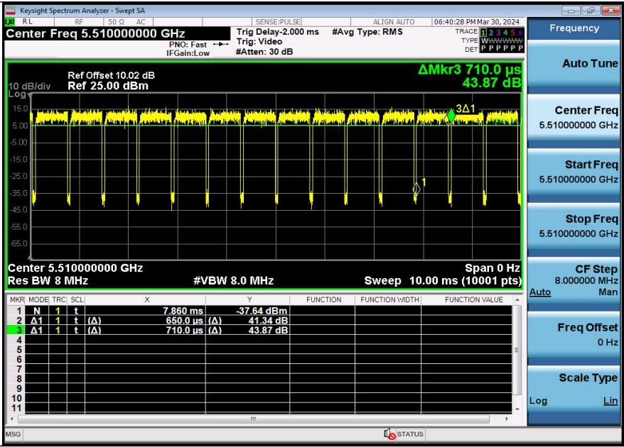
NTNV-11N40SISO-Ant3-5510
