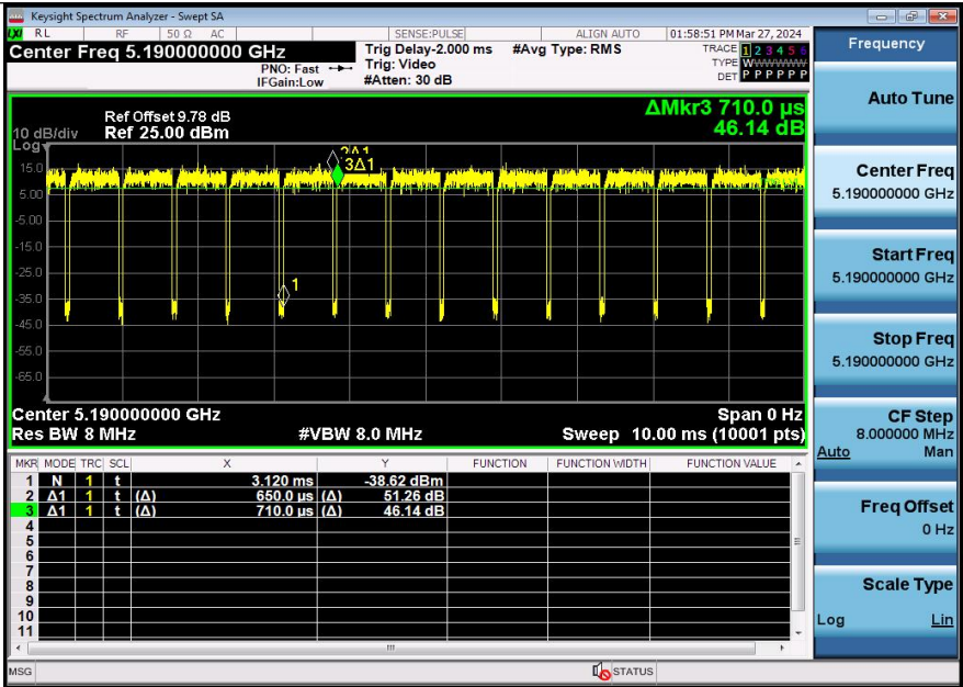
NTNV-11N40SISO-Ant3-5190
