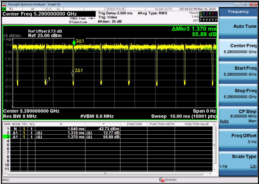
NTNV-11N20SISO-Ant3-5280
