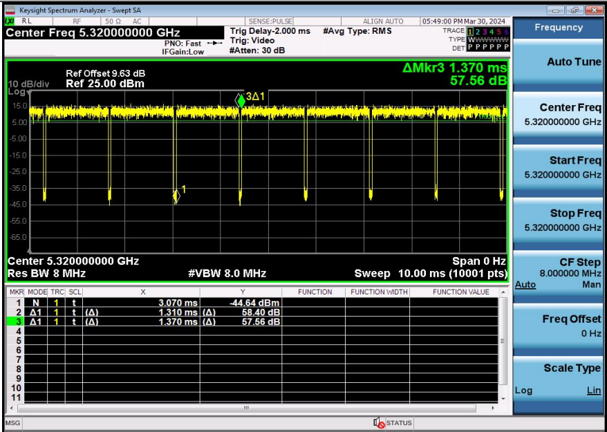
NTNV-11N20SISO-Ant3-5320
