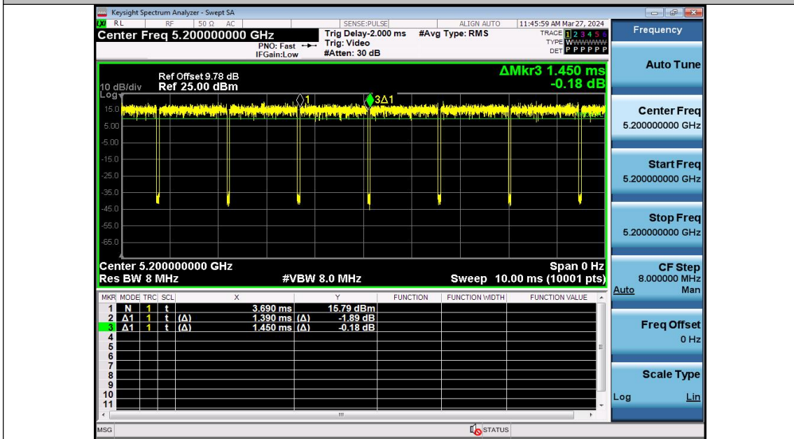
NTNV-11A-Ant3-5200
