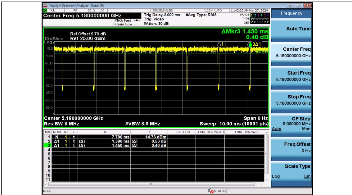
NTNV-11A-Ant3-5180
