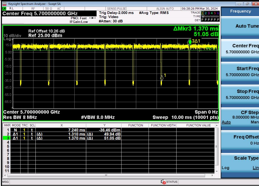
NTNV-11N20SISO-Ant3-5700
