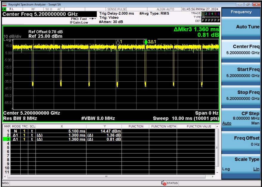
NTNV-11N20SISO-Ant3-5200
