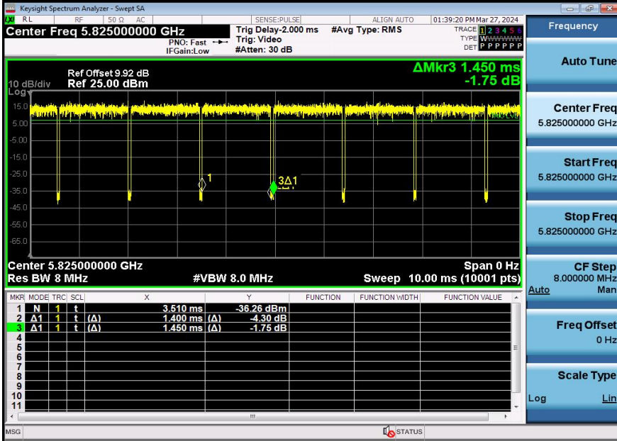
NTNV-11A-Ant3-5825
