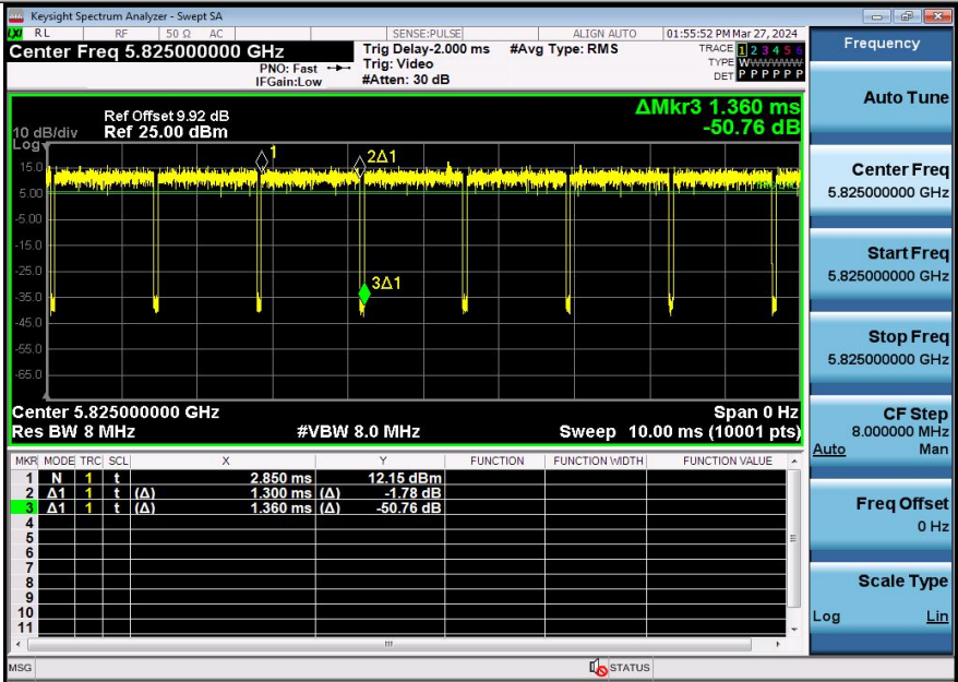
NTNV-11N20SISO-Ant3-5825
