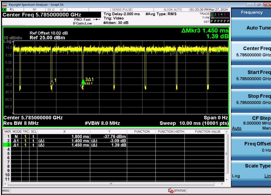
NTNV-11A-Ant3-5785
