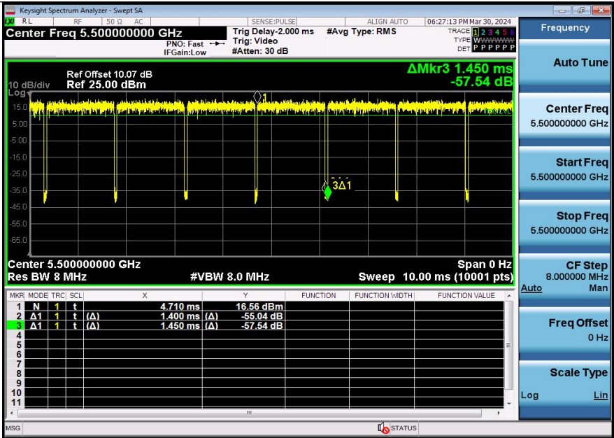
NTNV-11A-Ant3-5500
