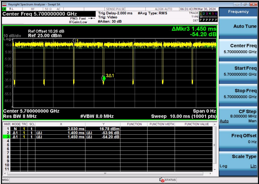
NTNV-11A-Ant3-5700
