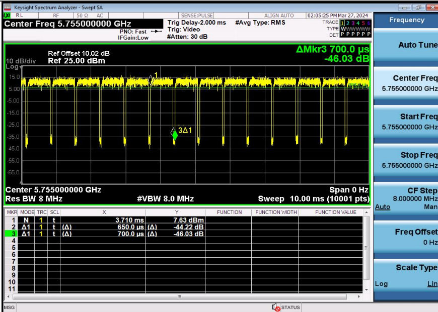
NTNV-11N40SISO-Ant3-5755
