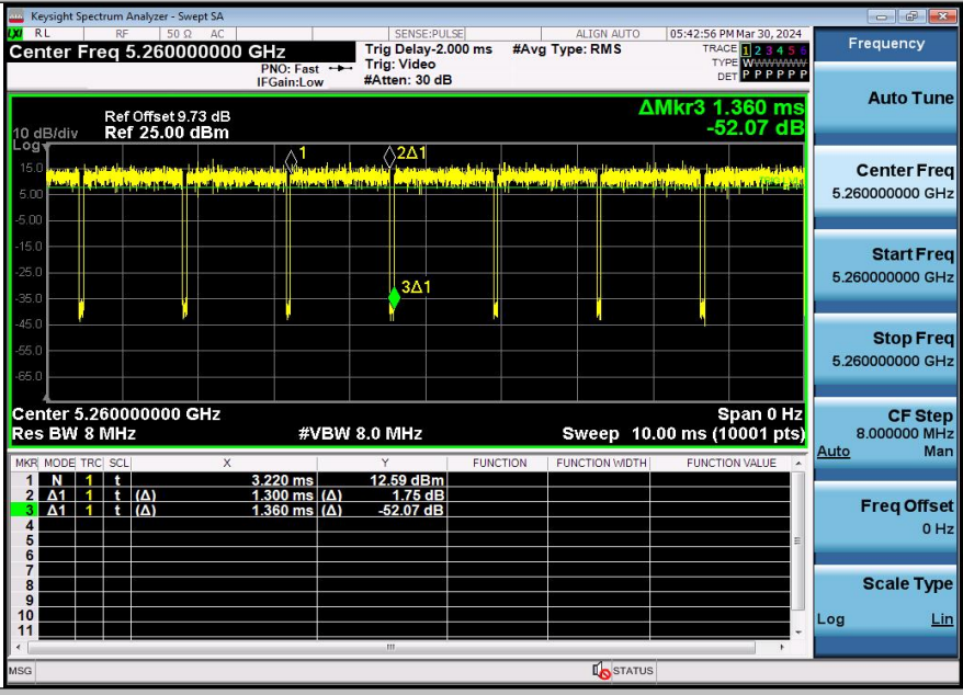
NTNV-11N20SISO-Ant3-5260
