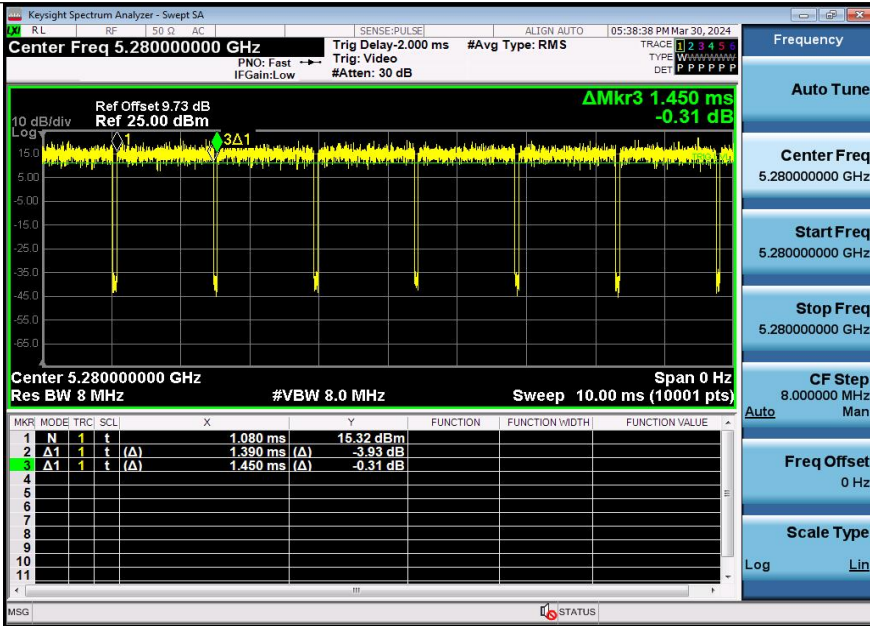
NTNV-11A-Ant3-5280
