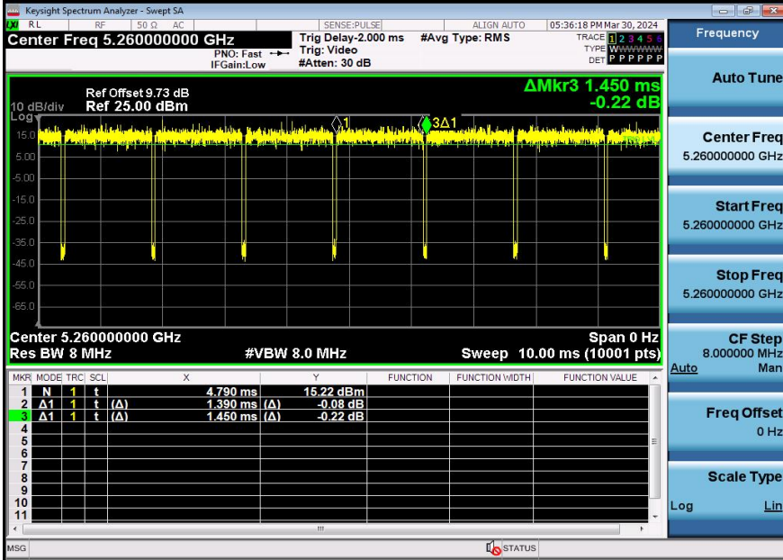
NTNV-11A-Ant3-5260
