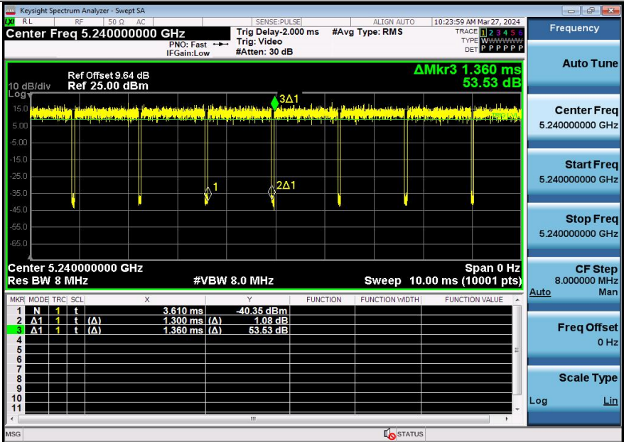
NTNV-11AC20SISO-Ant2-5240
