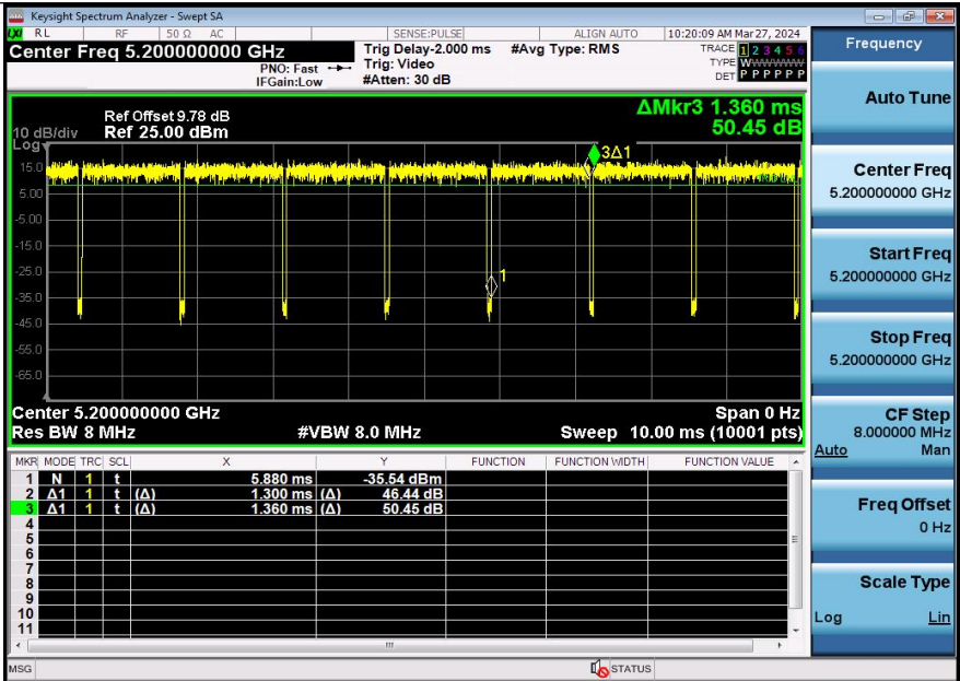
NTNV-11AC20SISO-Ant2-5200
