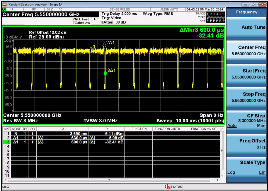
NTNV-11AC40SISO-Ant2-5550
