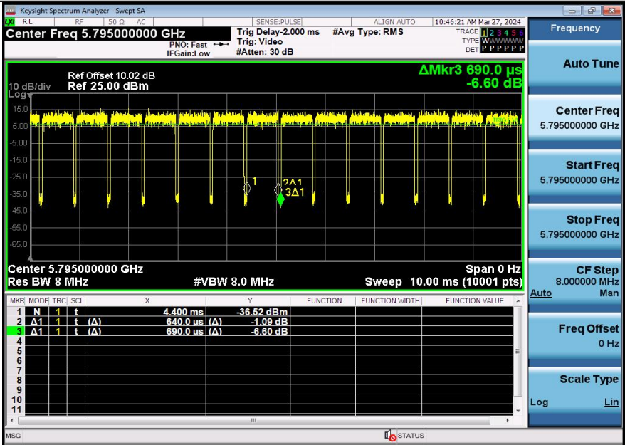
NTNV-11AC40SISO-Ant2-5795
