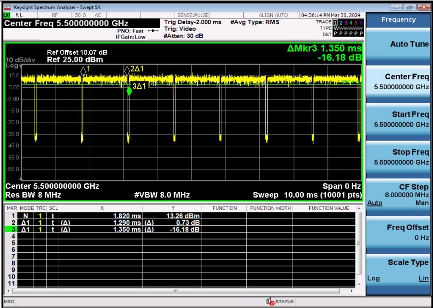
NTNV-11AC20SISO-Ant2-5500
