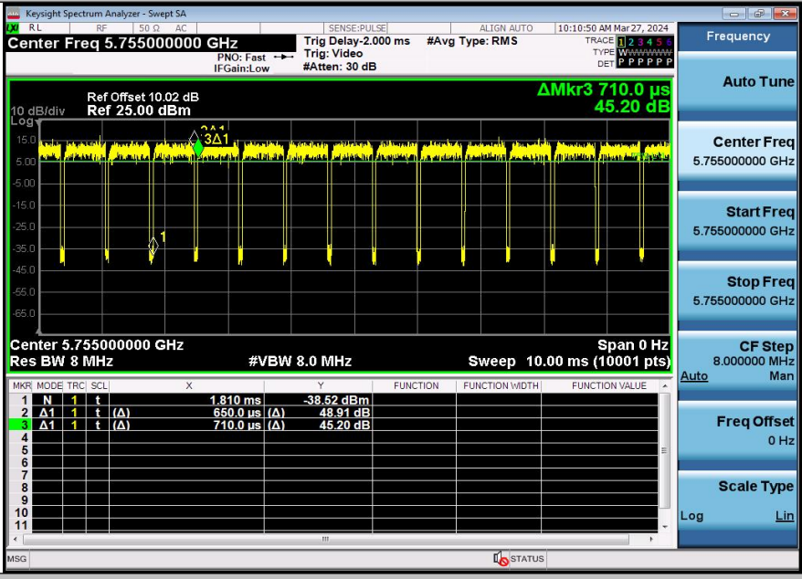
NTNV-11N40SISO-Ant2-5755
