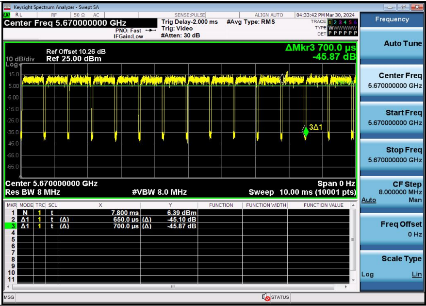
NTNV-11N40SISO-Ant2-5670
