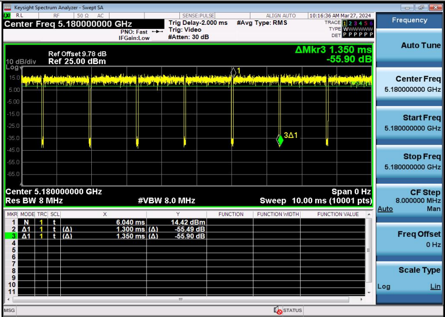
NTNV-11AC20SISO-Ant2-5180
