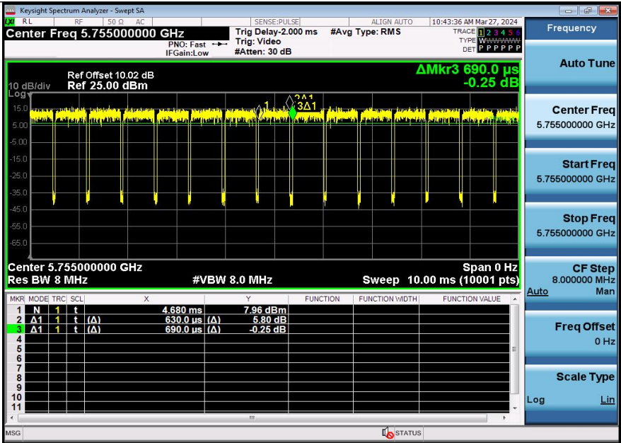
NTNV-11AC40SISO-Ant2-5755
