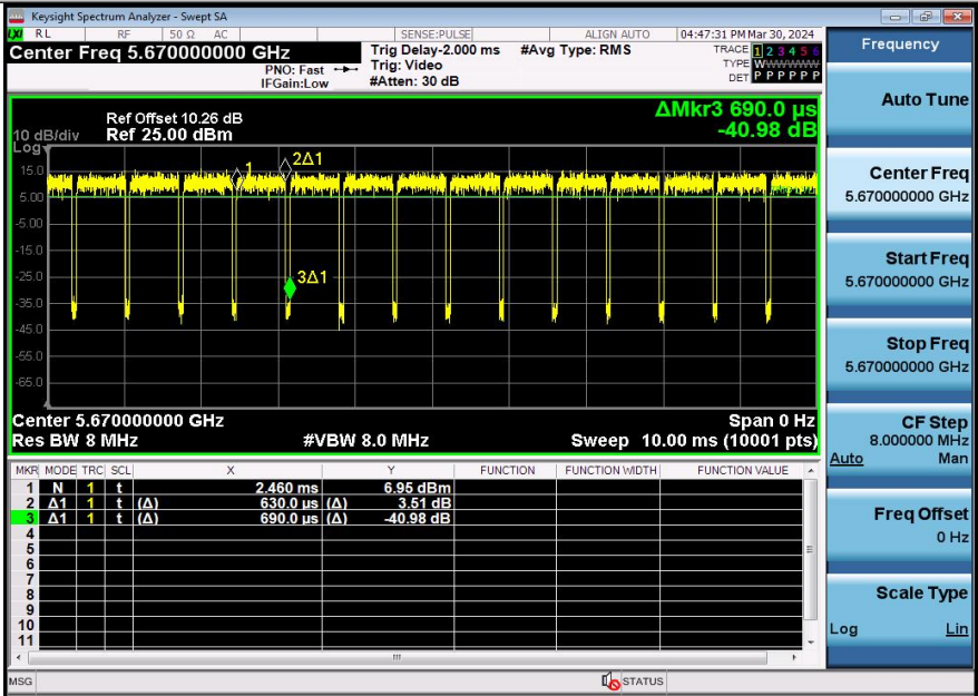
NTNV-11AC40SISO-Ant2-5670
