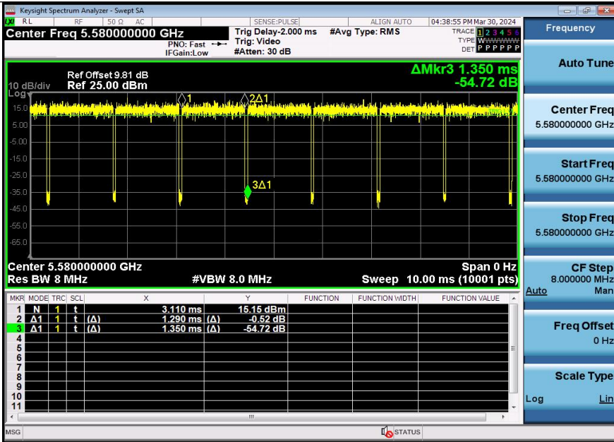
NTNV-11AC20SISO-Ant2-5580
