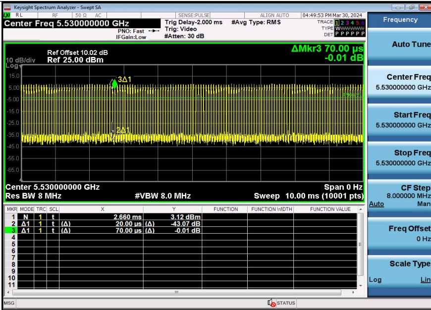
NTNV-11AC80SISO-Ant2-5530
