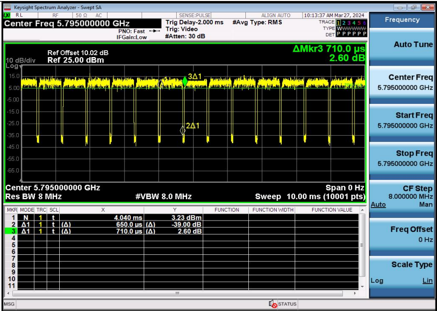
NTNV-11N40SISO-Ant2-5795
