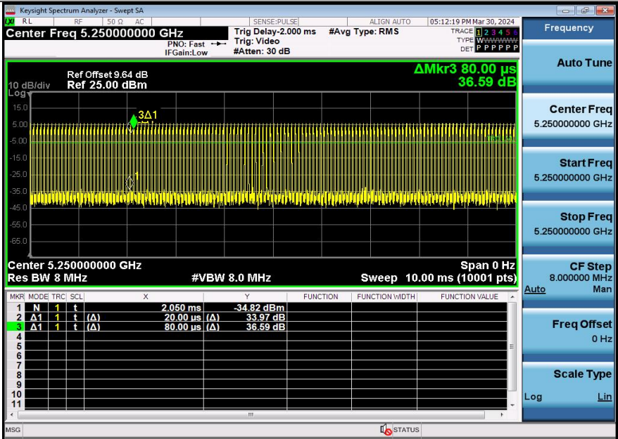
NTNV-11AC160SISO-Ant2-5250
