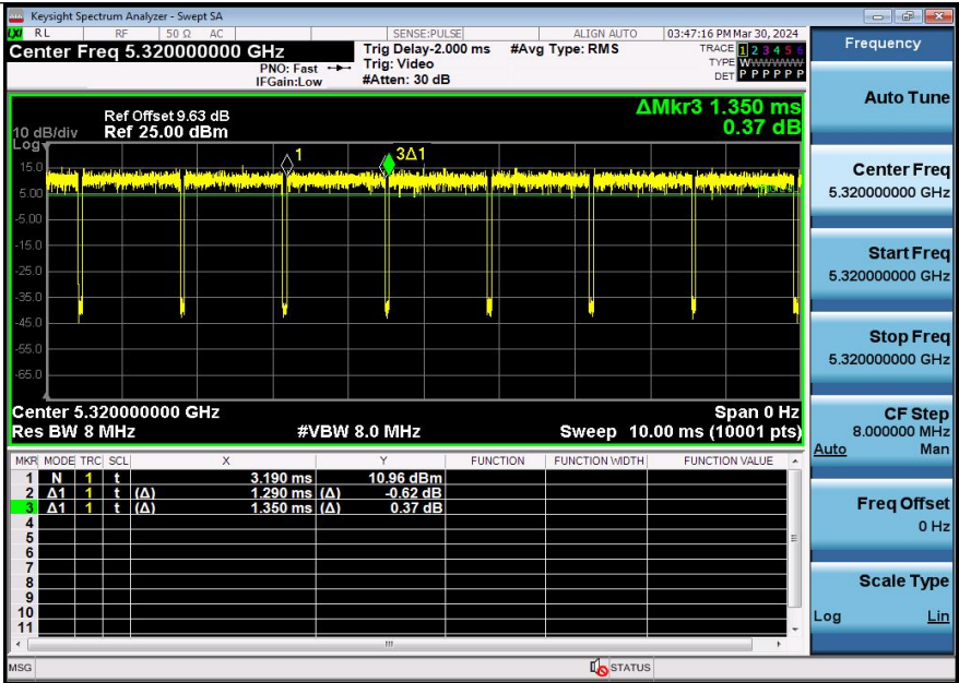
NTNV-11AC20SISO-Ant2-5320
