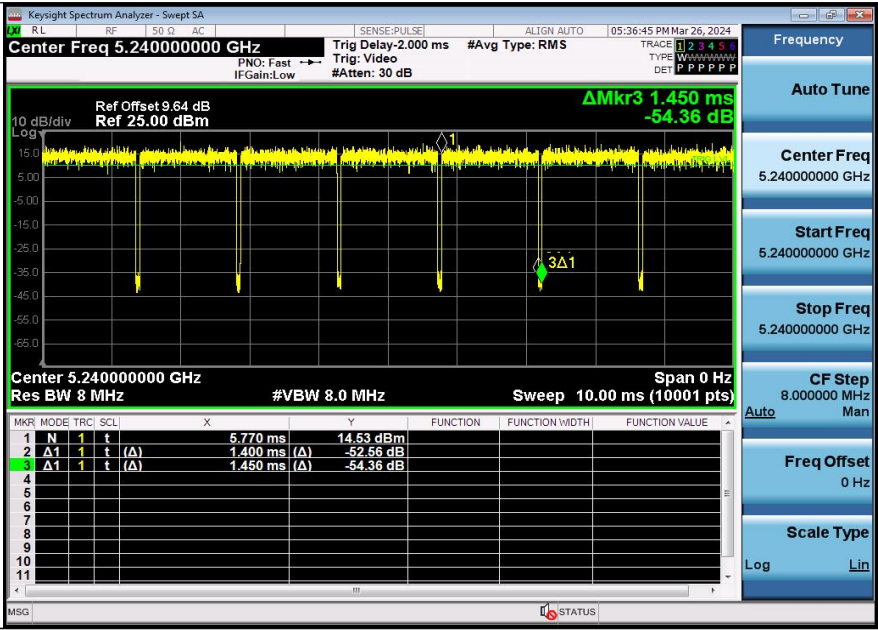
NTNV-11A-Ant2-5240
