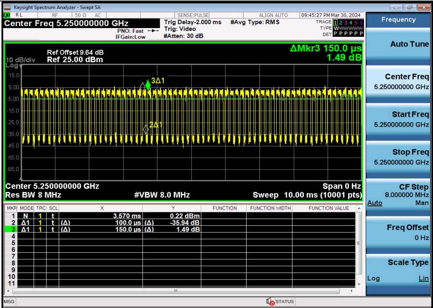
NTNV-11AX160SISO-Ant1-5250
