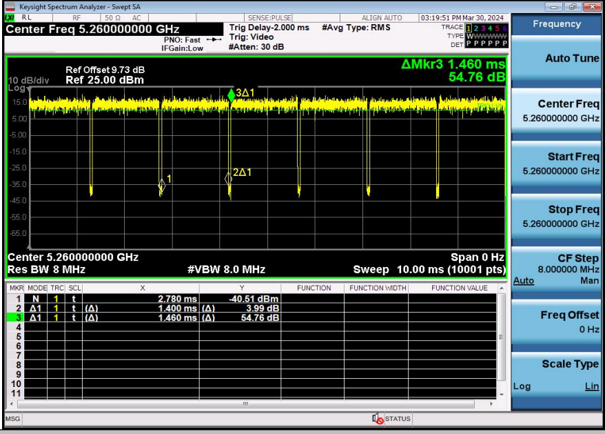
NTNV-11A-Ant2-5260
