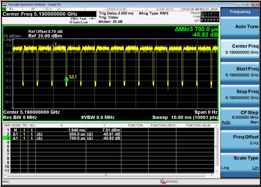
NTNV-11N40SISO-Ant2-5190
