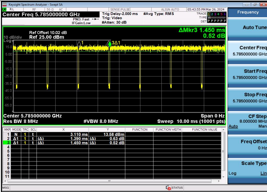
NTNV-11A-Ant2-5785
