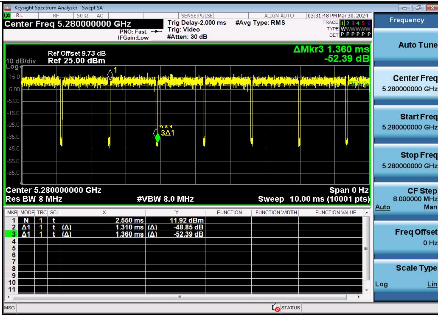
NTNV-11N20SISO-Ant2-5280
