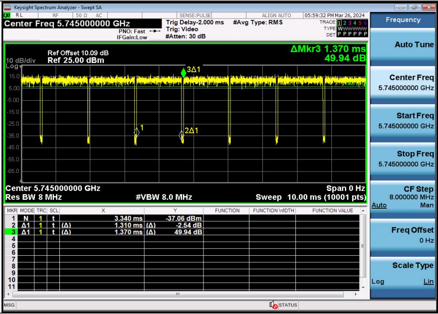
NTVN-11N20SISO-Ant2-5745
