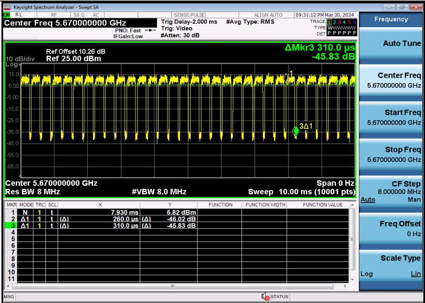
NTNV-11AX40SISO-Ant1-5670
