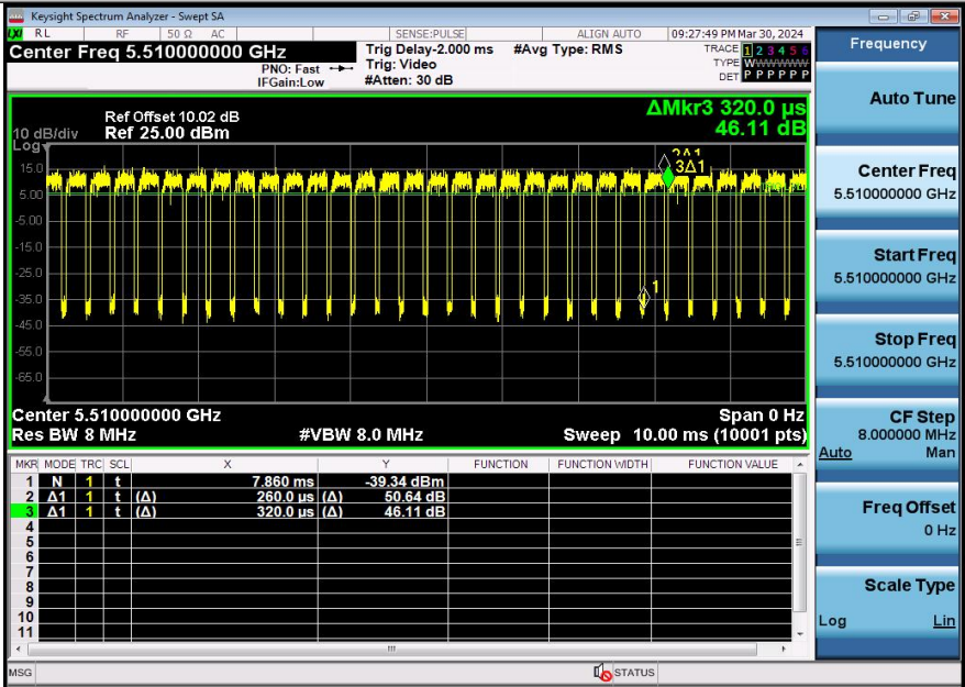
NTV-11AX40SISO-Ant1-5510
