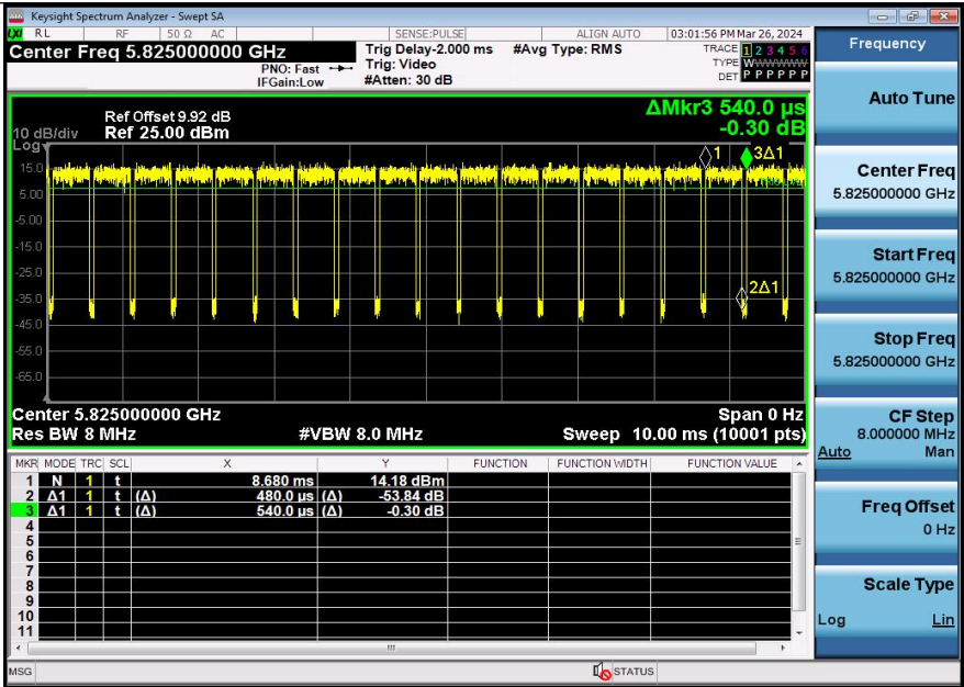
NTNV-11AX20SISO-Ant1-5825
