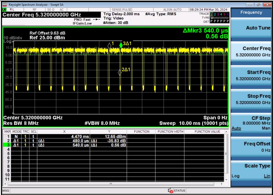
NTNV-11AX20SISO-Ant1-5320
