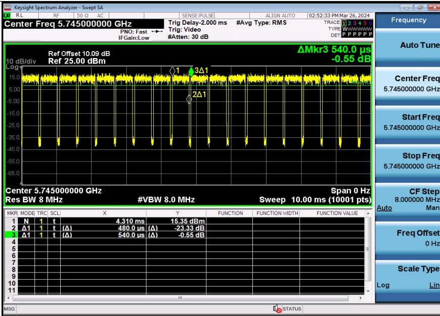
NTNV-11AX20SISO-Ant1-5745
