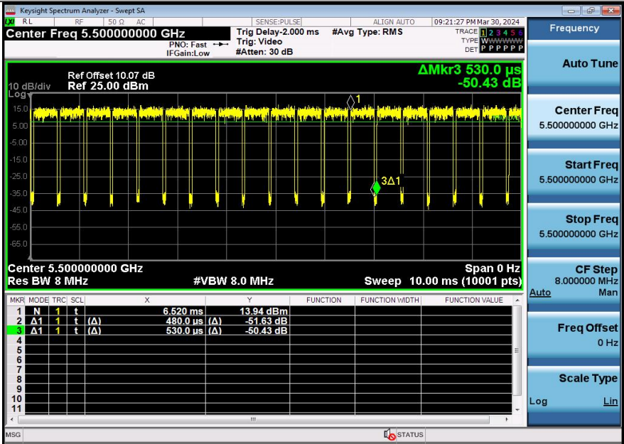
NTNV-11AX20SISO-Ant1-5500
