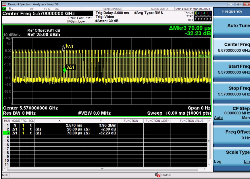
NTNV-11AC160SISO-Ant1-5570
