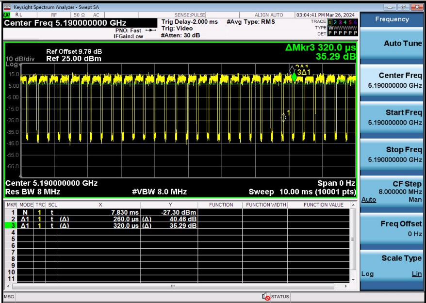
NTNV-11AX40SISO-Ant1-5190
