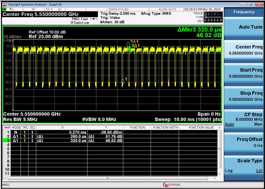
NTNV-11AX40SISO-Ant1-5550
