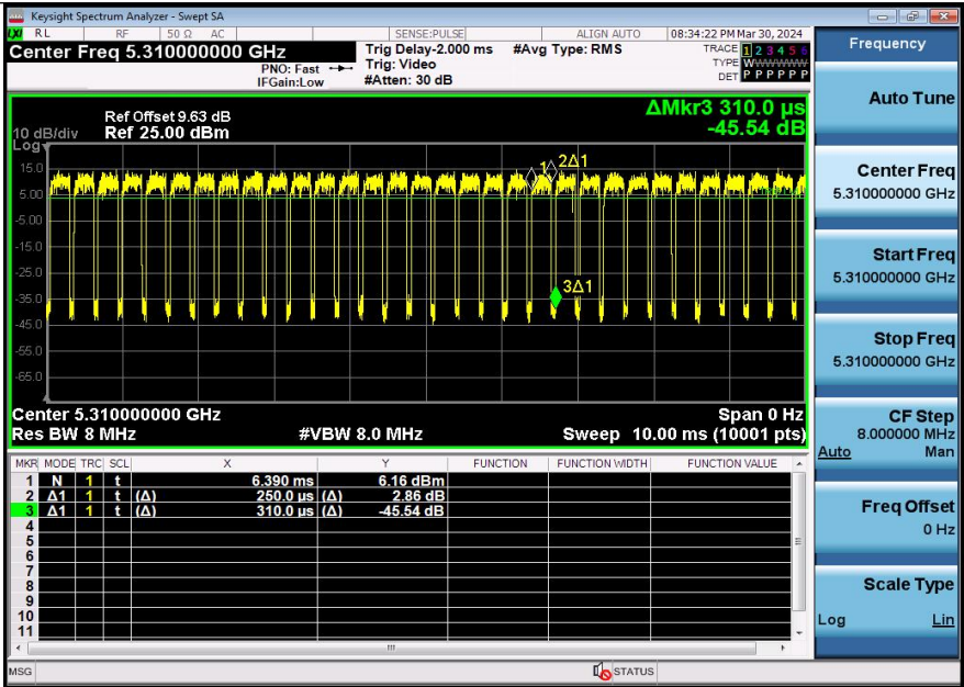
NTV-11AX40SISO-Ant1-5310
