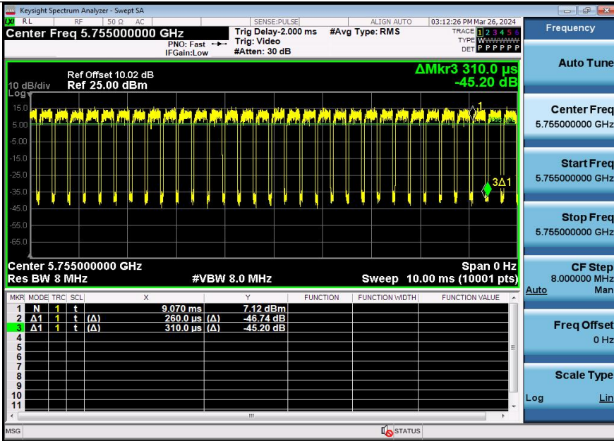
NTNV-11AX40SISO-Ant1-5755
