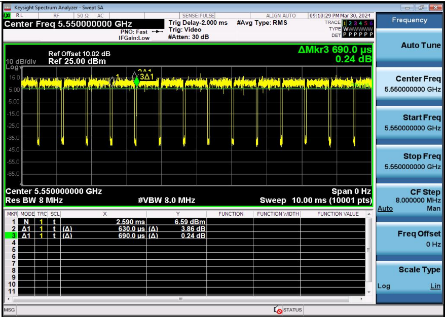
NTNV-11AC40SISO-Ant1-5550
