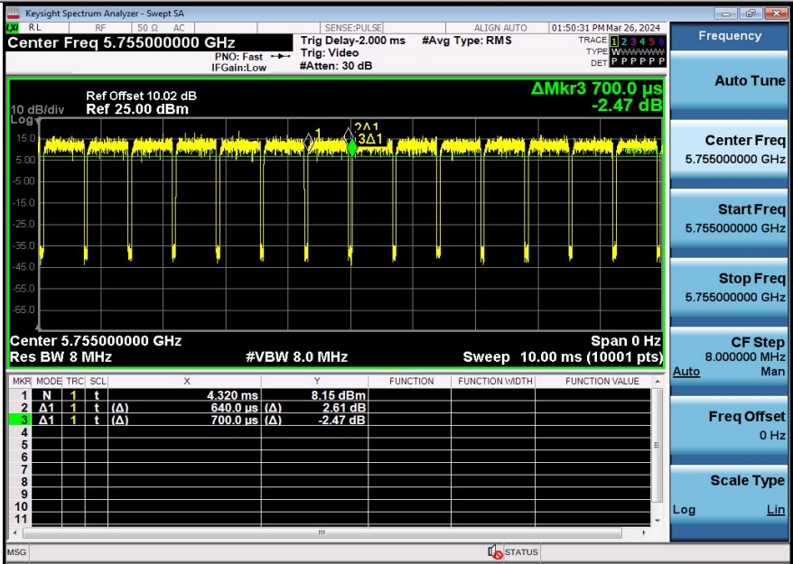
NTNV-11N40SISO-Ant1-5755
