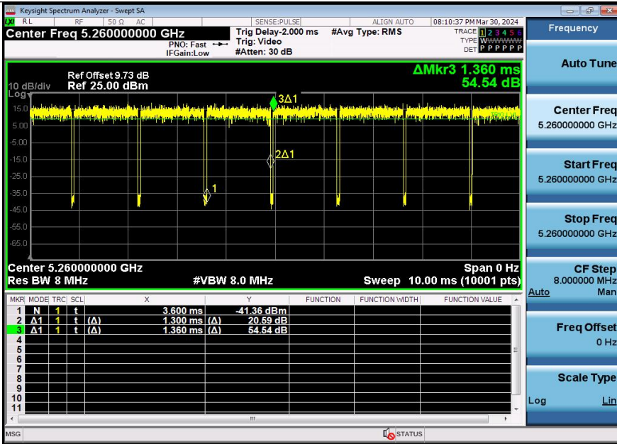
NTNV-11AC20SISO-Ant1-5260
