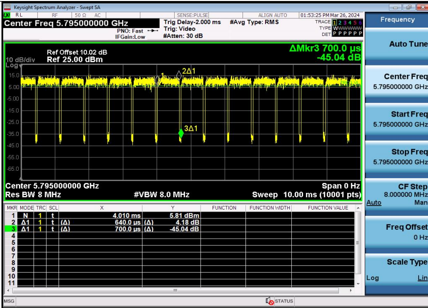
NTNV-11N40SISO-Ant1-5795
