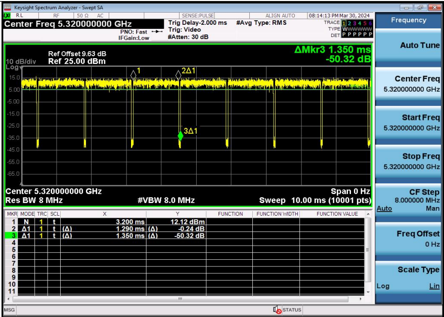
NTNV-11AC20SISO-Ant1-5320
