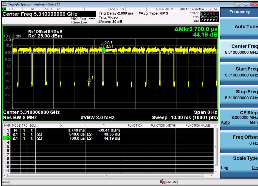
NTNV-11AC40SISO-Ant1-5310
