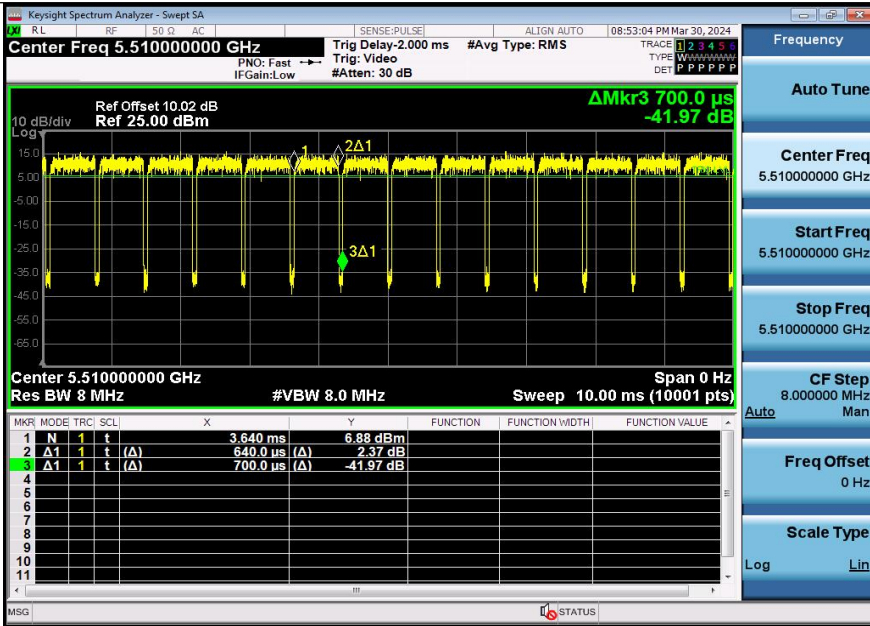
NTNV-11N40SISO-Ant1-5510
