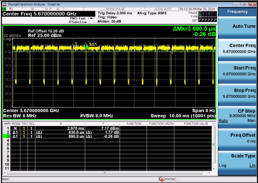
NTNV-11AC40SISO-Ant1-5670
