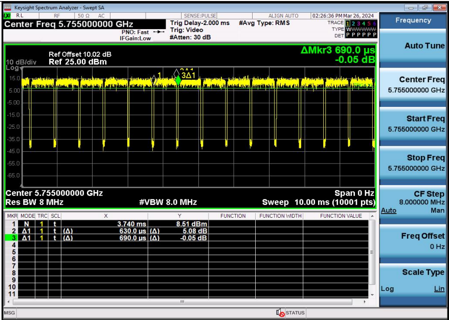
NTNV-11AC40SISO-Ant1-5755
