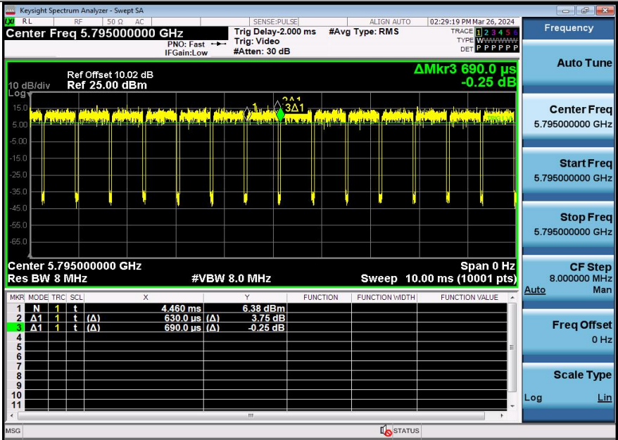
NTNV-11AC40SISO-Ant1-5795
