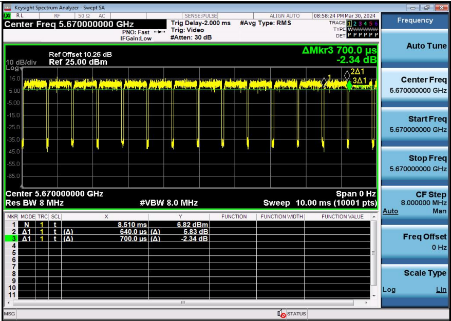
NTNV-11N40SISO-Ant1-5670
