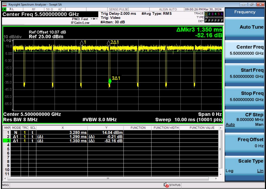
NTNV-11AC20SISO-Ant1-5500
