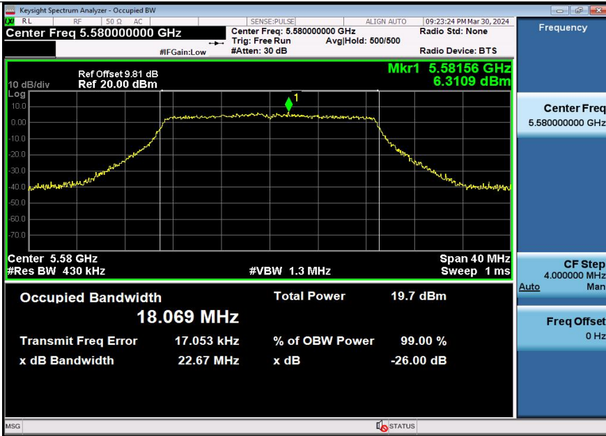
11AX20SISO-Ant1-5580
