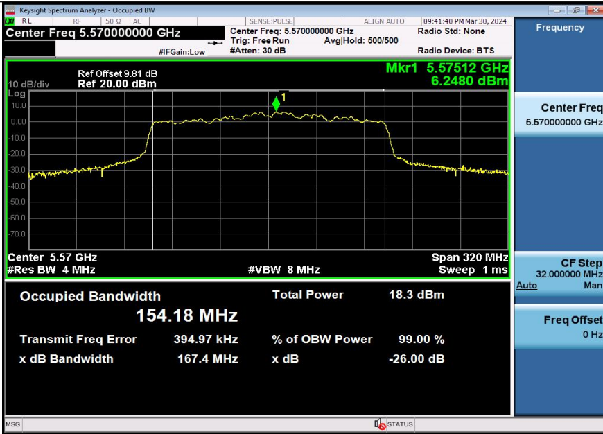
11AC160SISO-Ant1-5570
