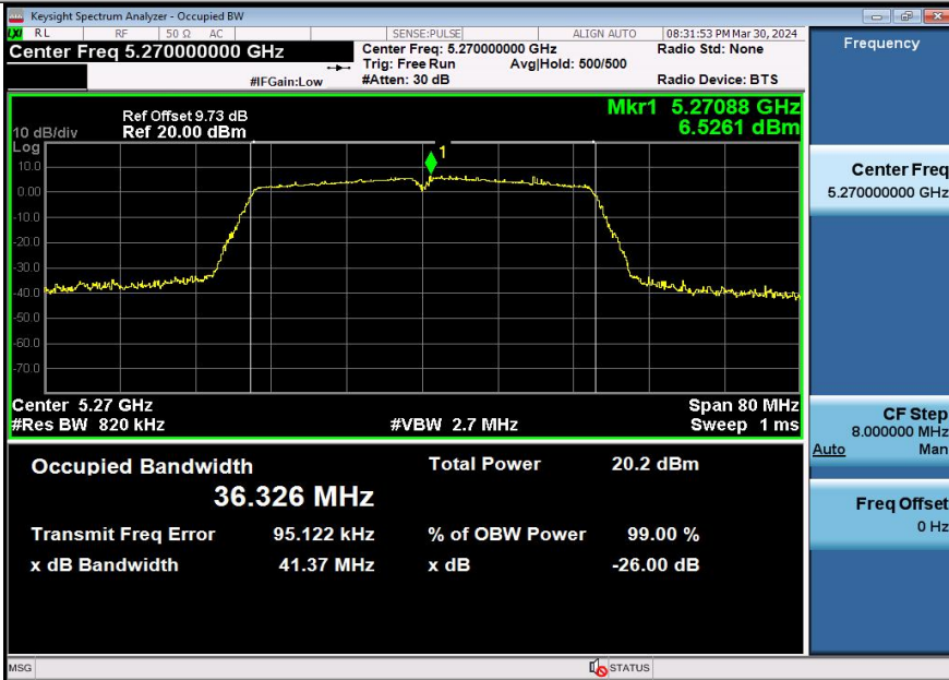
11AX40SISO-Ant1-5270
