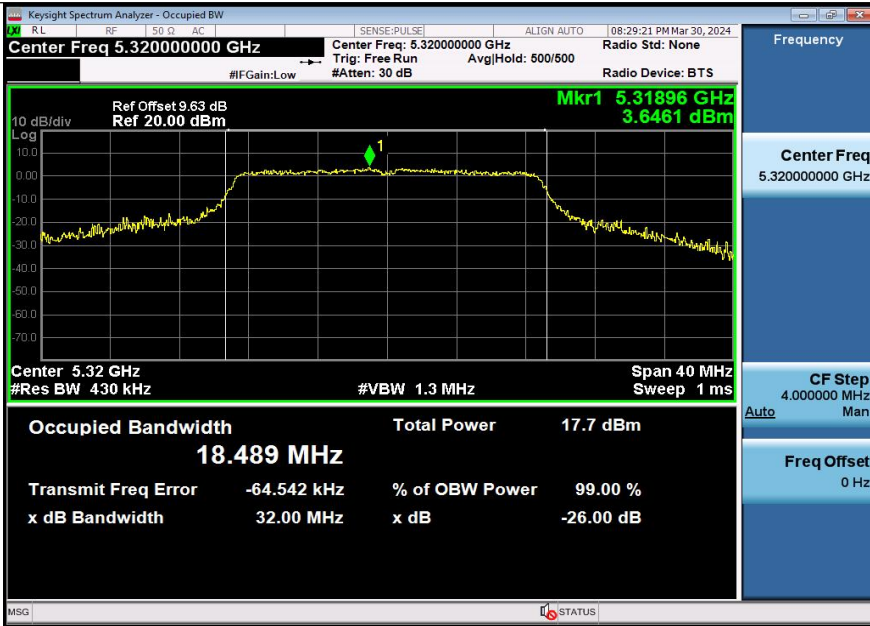
11AX20SISO-Ant1-5320
