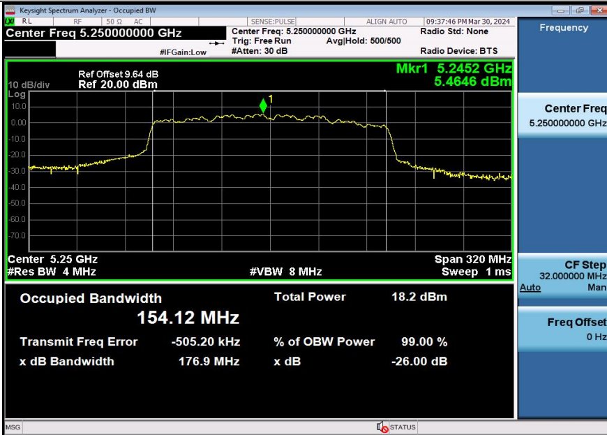
11AC160SISO-Ant1-5250
