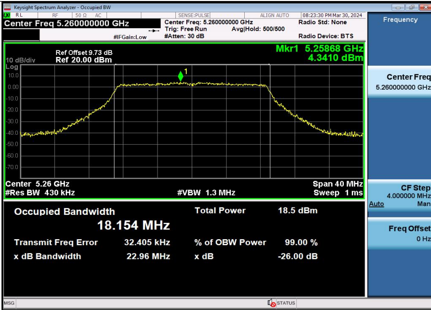
11AX20SISO-Ant1-5260
