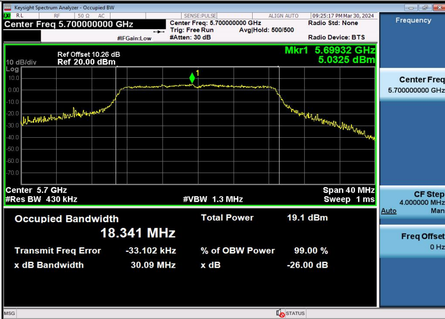
11AX20SISO-Ant1-5700
