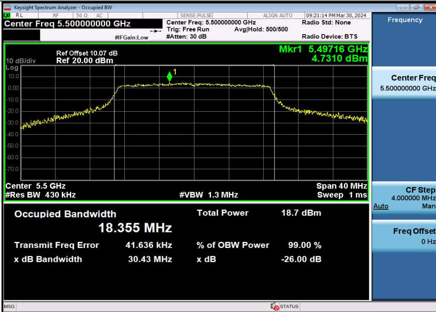
11AX20SISO-Ant1-5500
