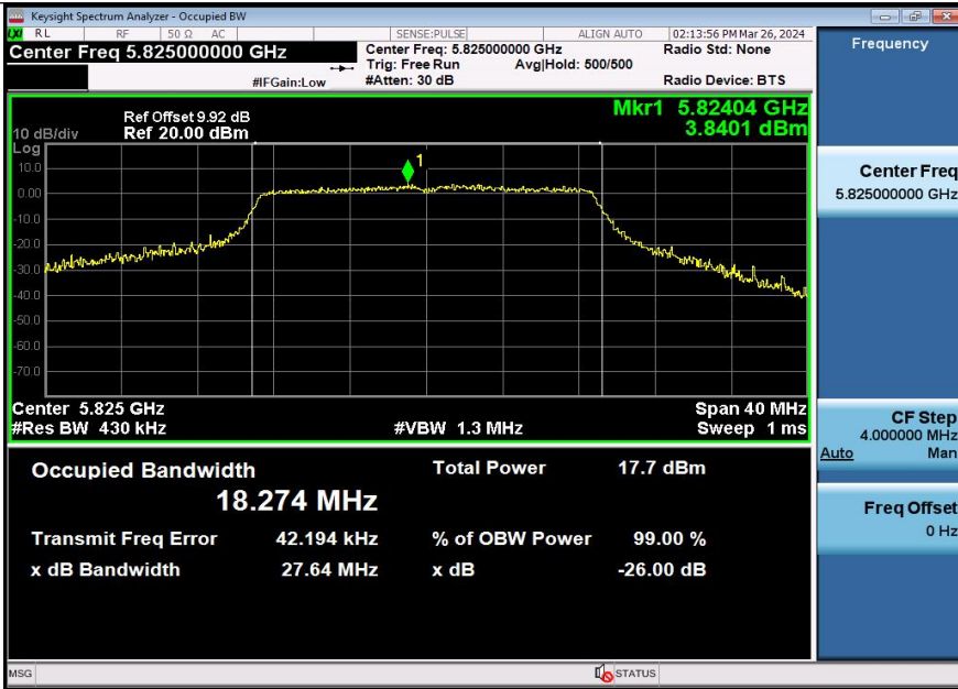
11AC20SISO-Ant1-5825
