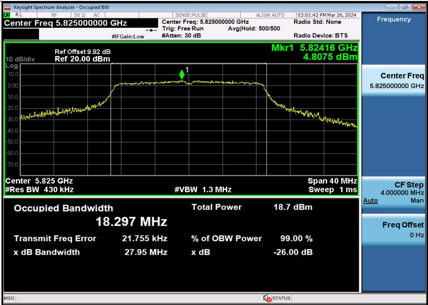
11AX20SISO-Ant1-5825
