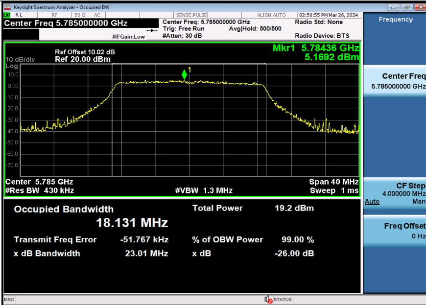
11AX20SISO-Ant1-5785
