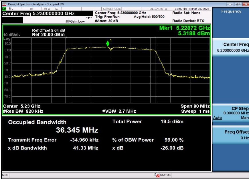
11AX40SISO-Ant1-5230
