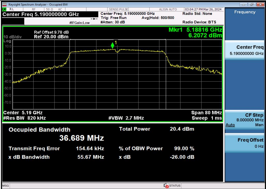
11AX40SISO-Ant1-5190
